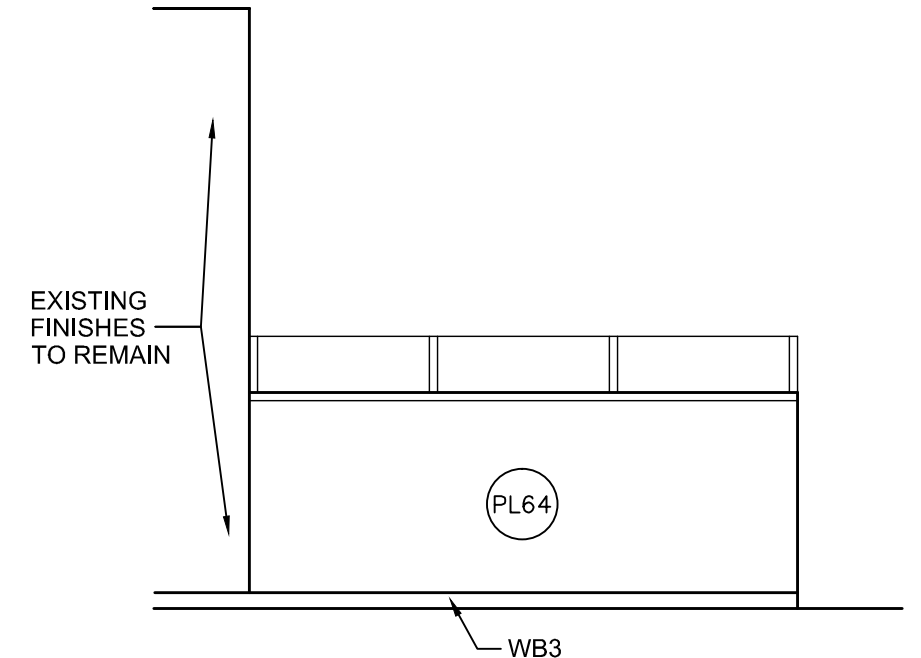
P CAFE 1/4" = 1'-0"
