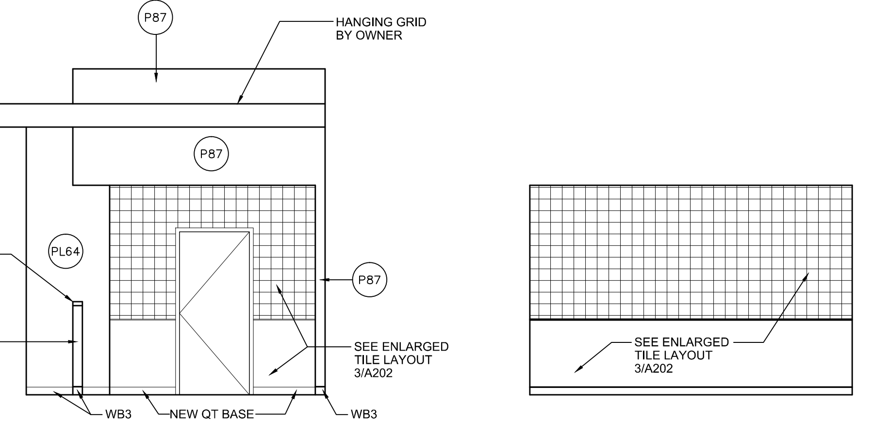
C BEVERAGE CENTER 1/4" = 1'-0"
