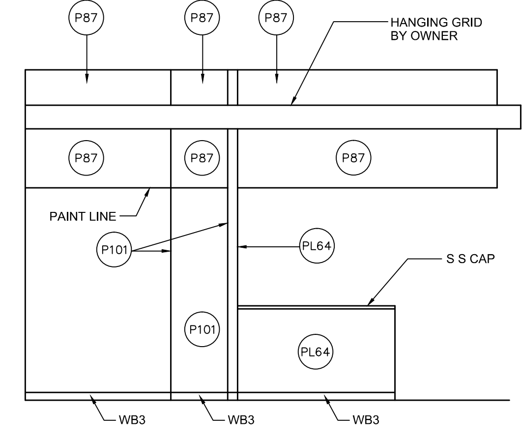
E BEVERAGE CENTER 1/4" = 1'-0"
