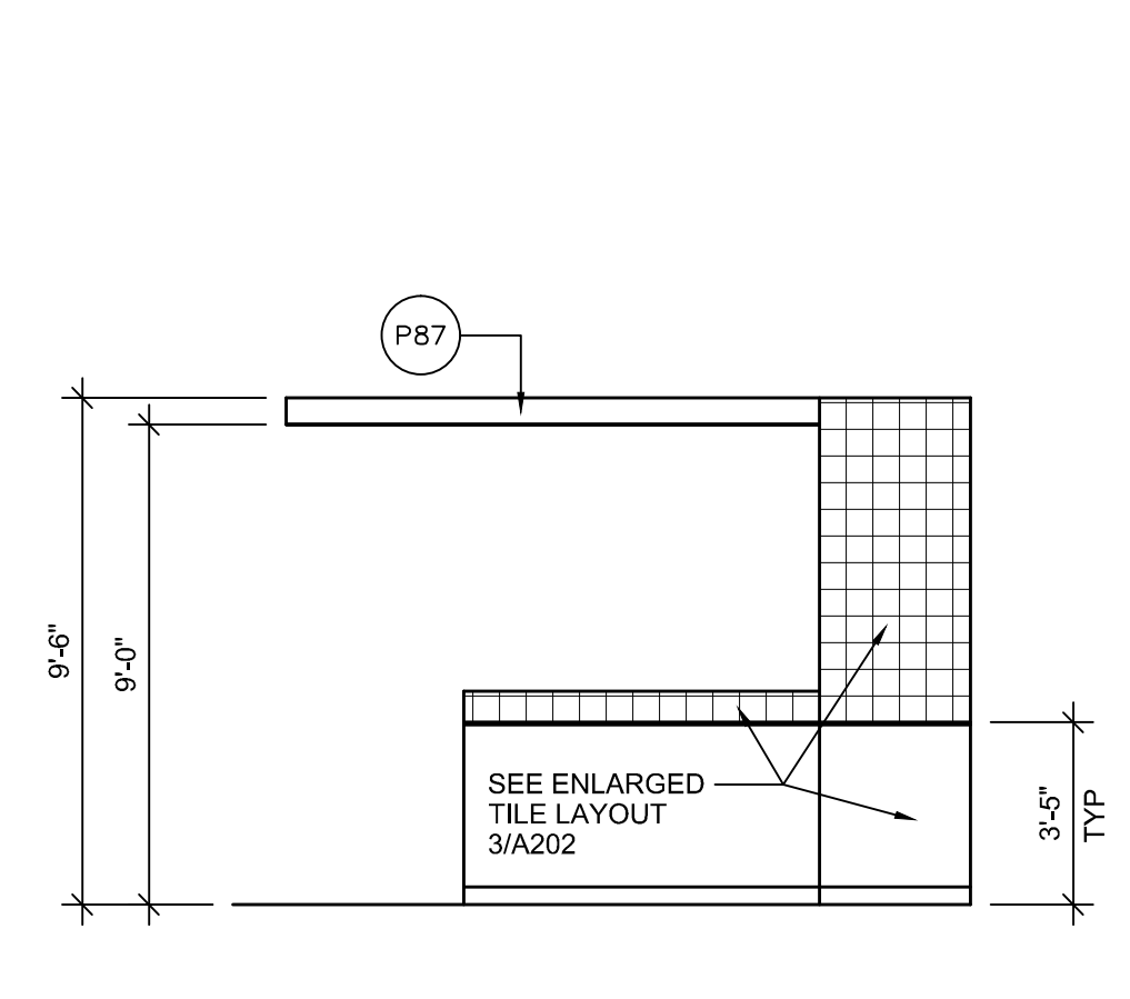
D BEVERAGE CENTER 1/4" = 1'-0"
