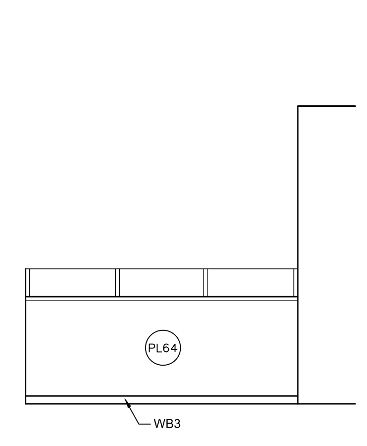
G CAFE 1/4" = 1'-0"
