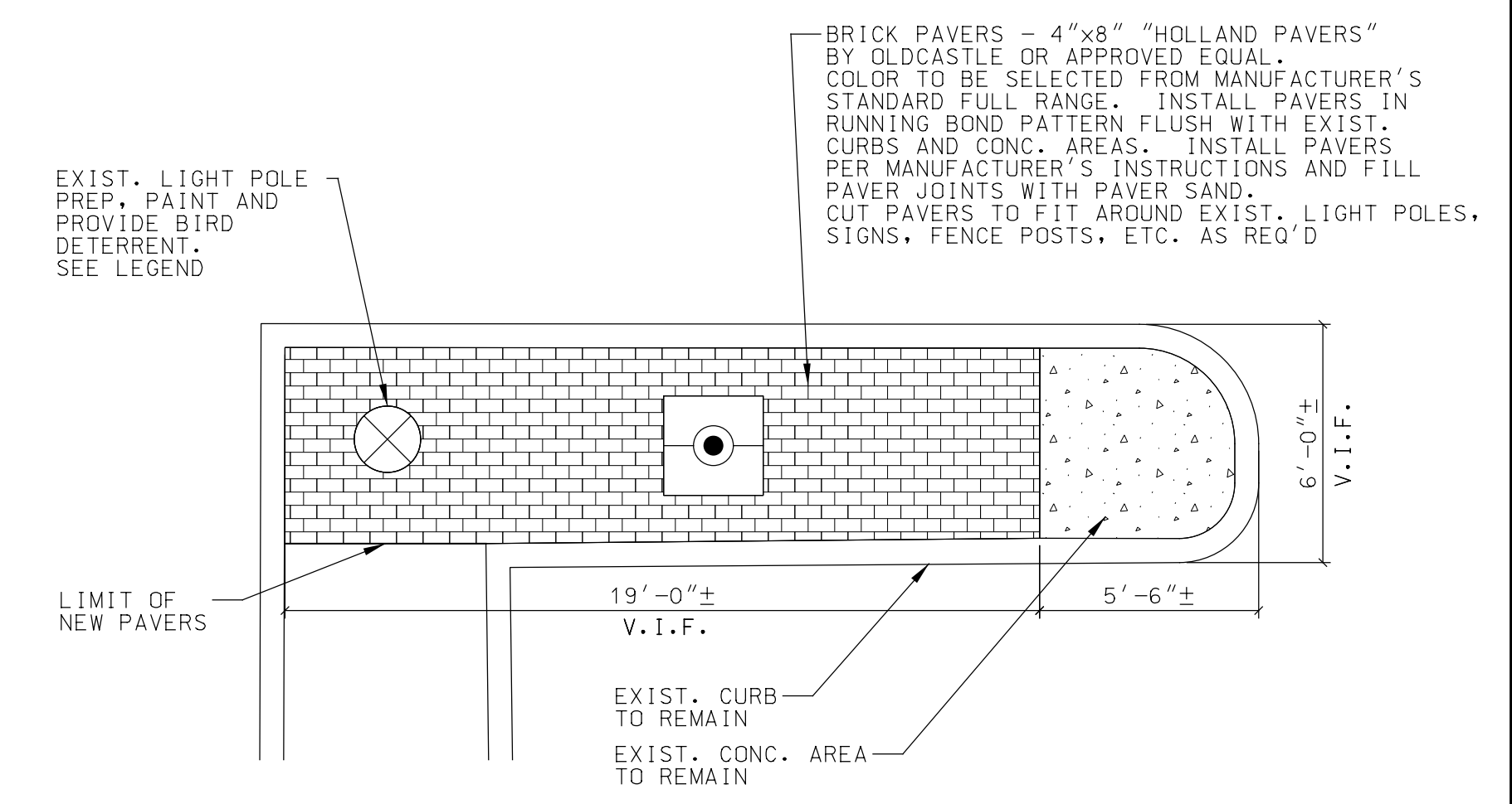
D2 ENLARGED PLAN A002 1/4" = 1'-0"
