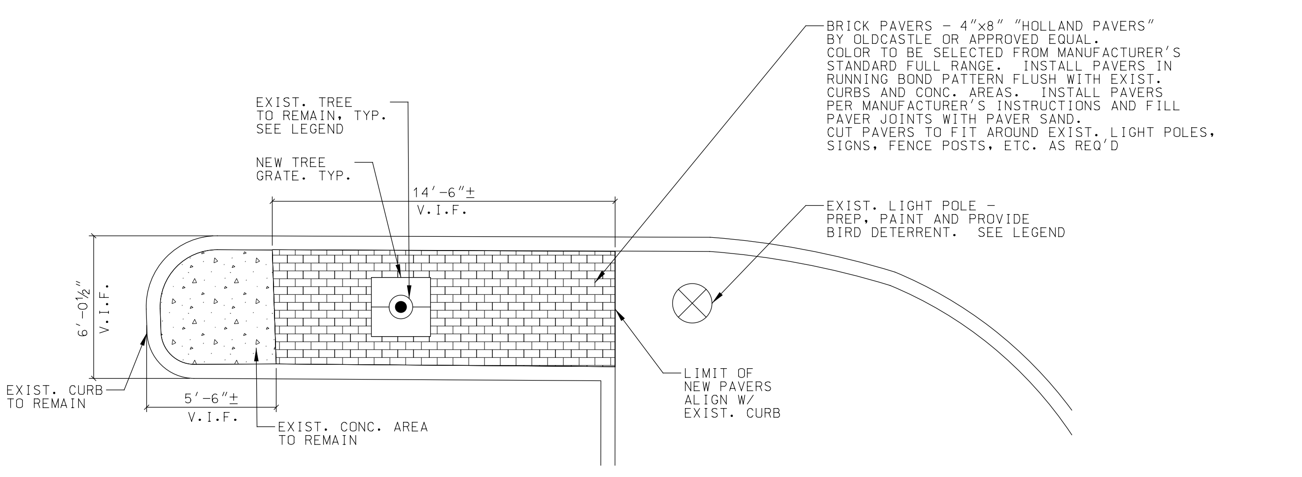
E1 ENLARGED PLAN A002 1/4" = 1'-0"
