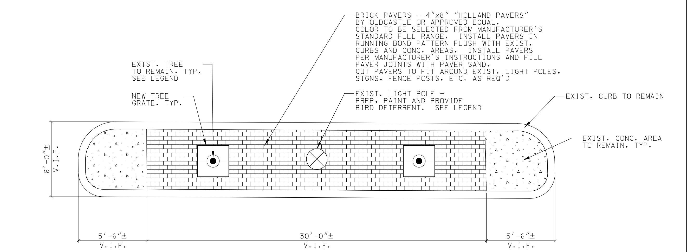
E2 ENLARGED PLAN A002 1/4" = 1'-0"
