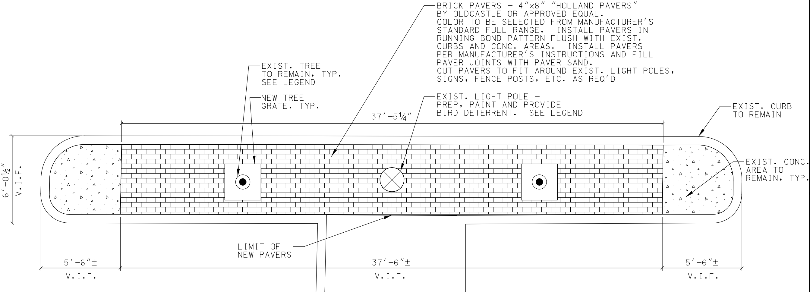
E3 ENLARGED PLAN A002 1/4" = 1'-0"
