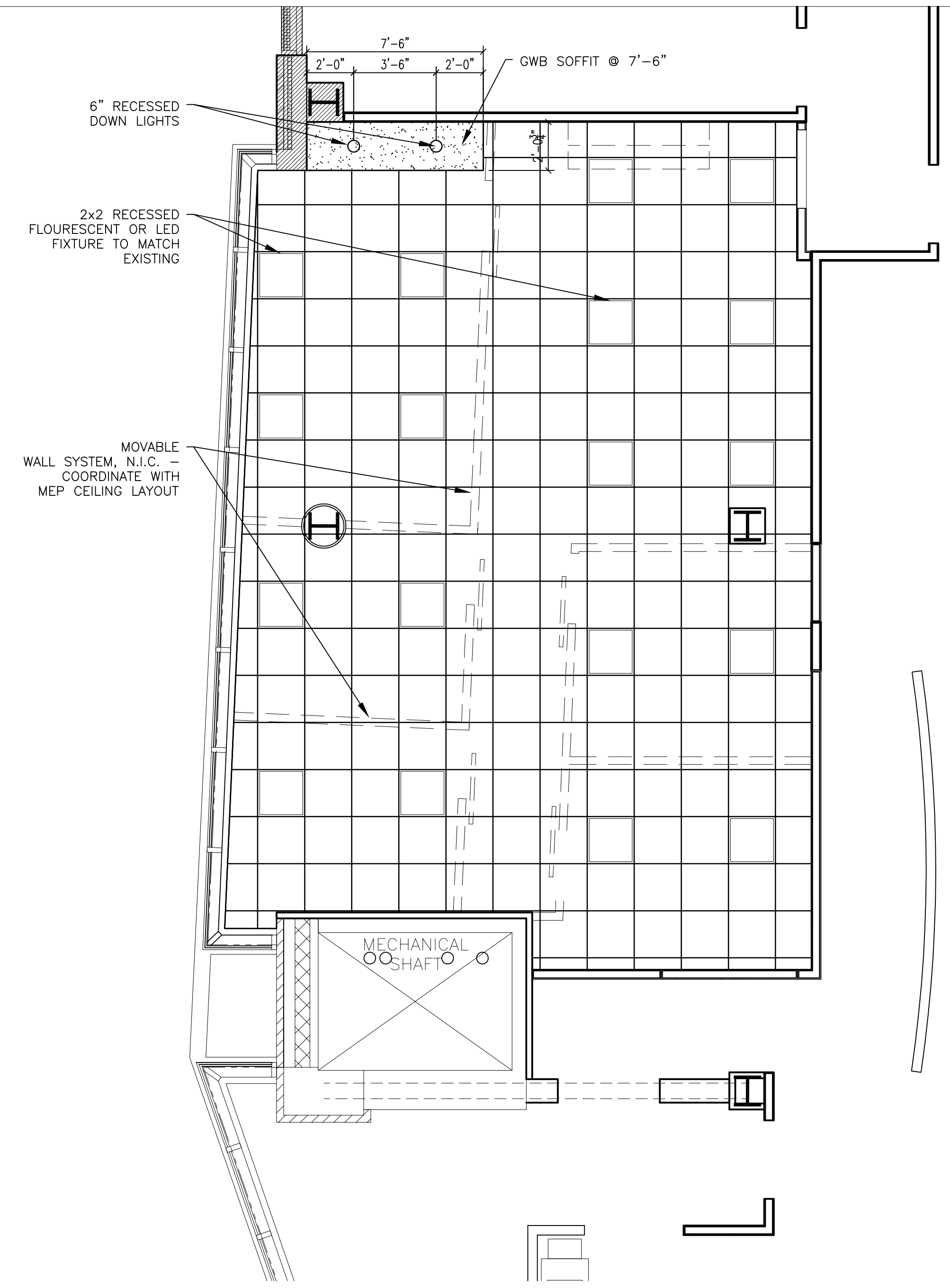
1 REFLECTED CEILING PLAN 1/8" = 1'-0"
