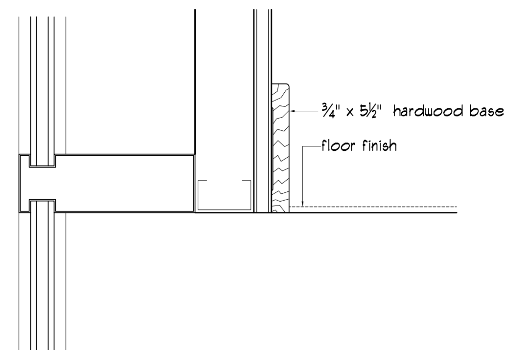
1 detail at exterior wall scale: 3"= 1'-0"
