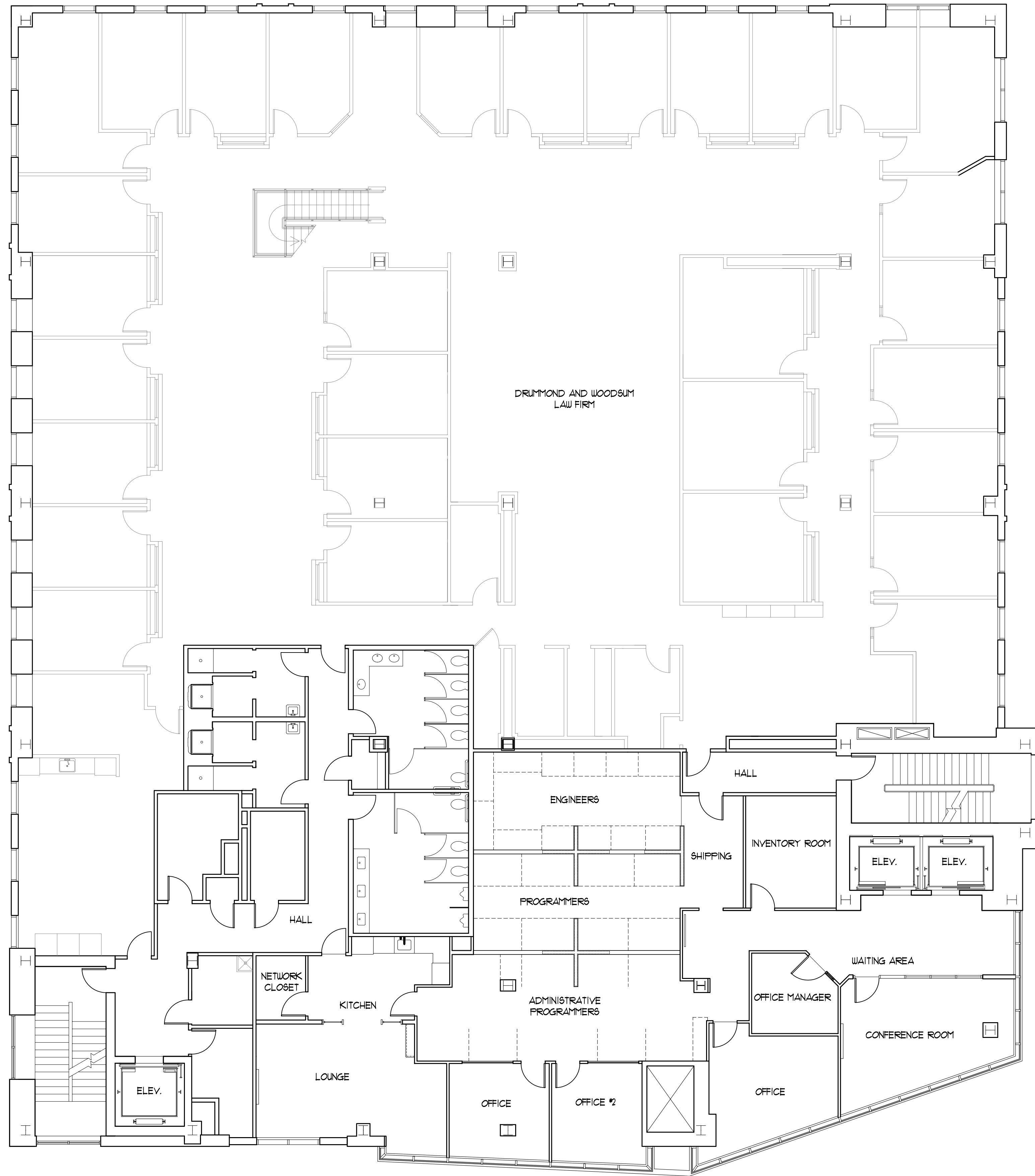
1 5th floor plan scale: 1/8" = 1'-0"
