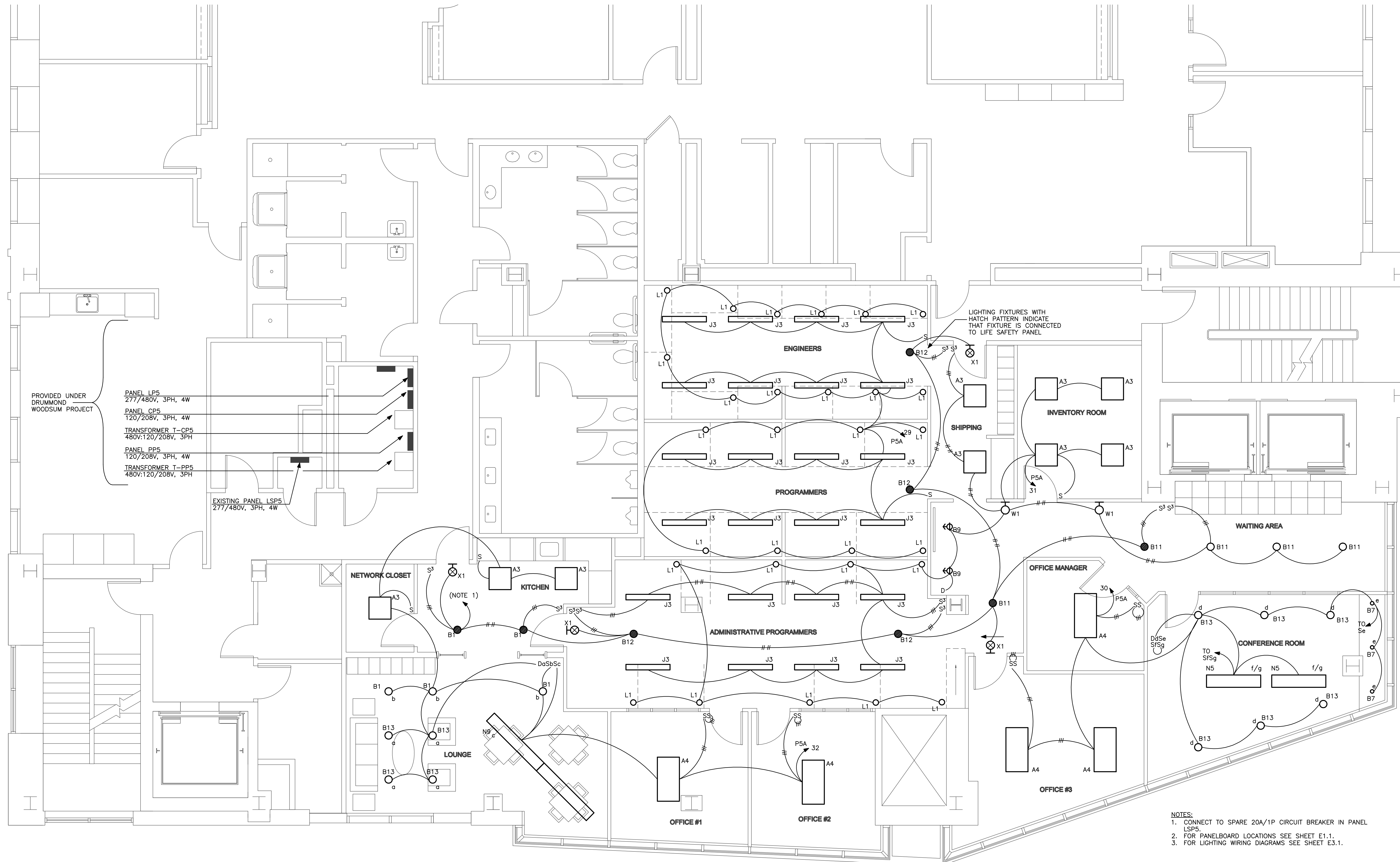
LIGHTING PLAN 1/4" = 1'-0"
