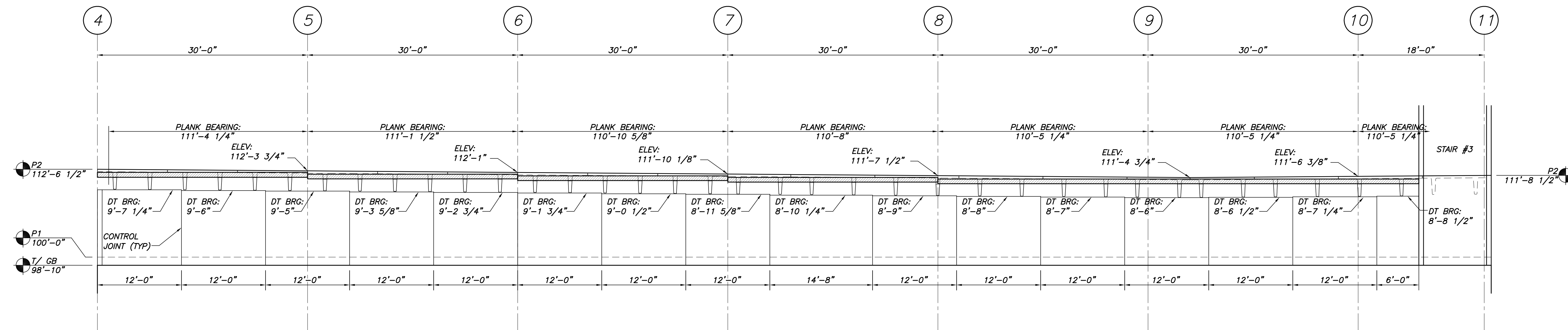
CMU WALL ELEVATION ALONG B.4 LINE 1/8"=1'-0"
