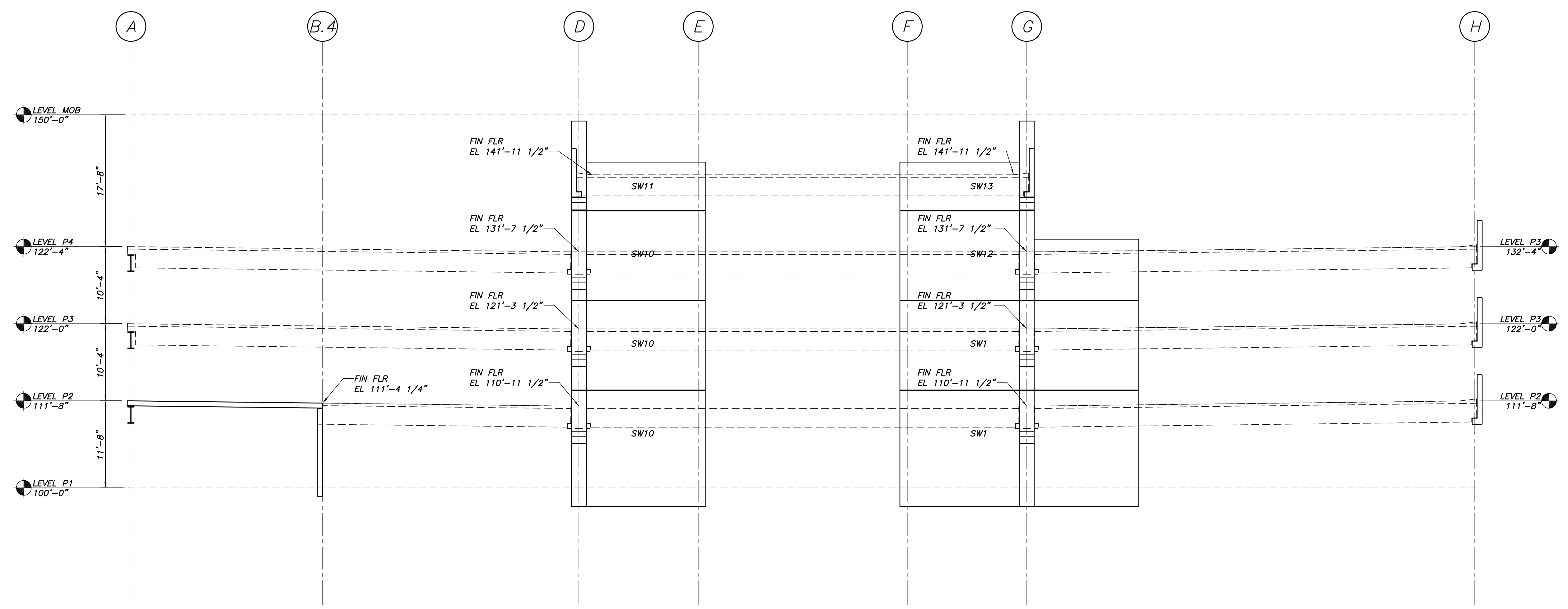
LITE WALL ELEVATION ALONG "9.2" LINE 1/8"=1'-0"
