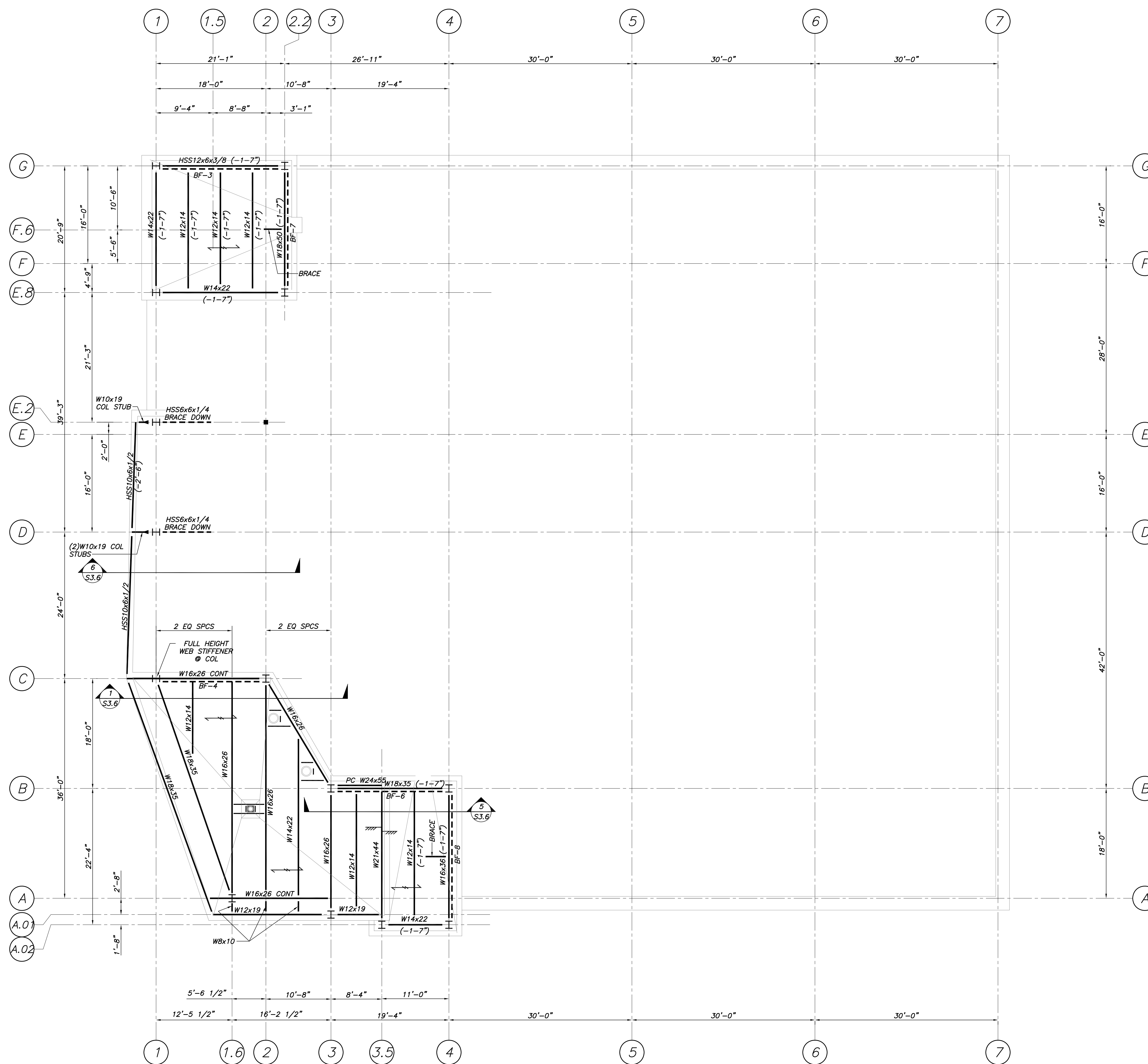
PENTHOUSE ROOF FRAMING PLAN 1/8"=1'-0"
