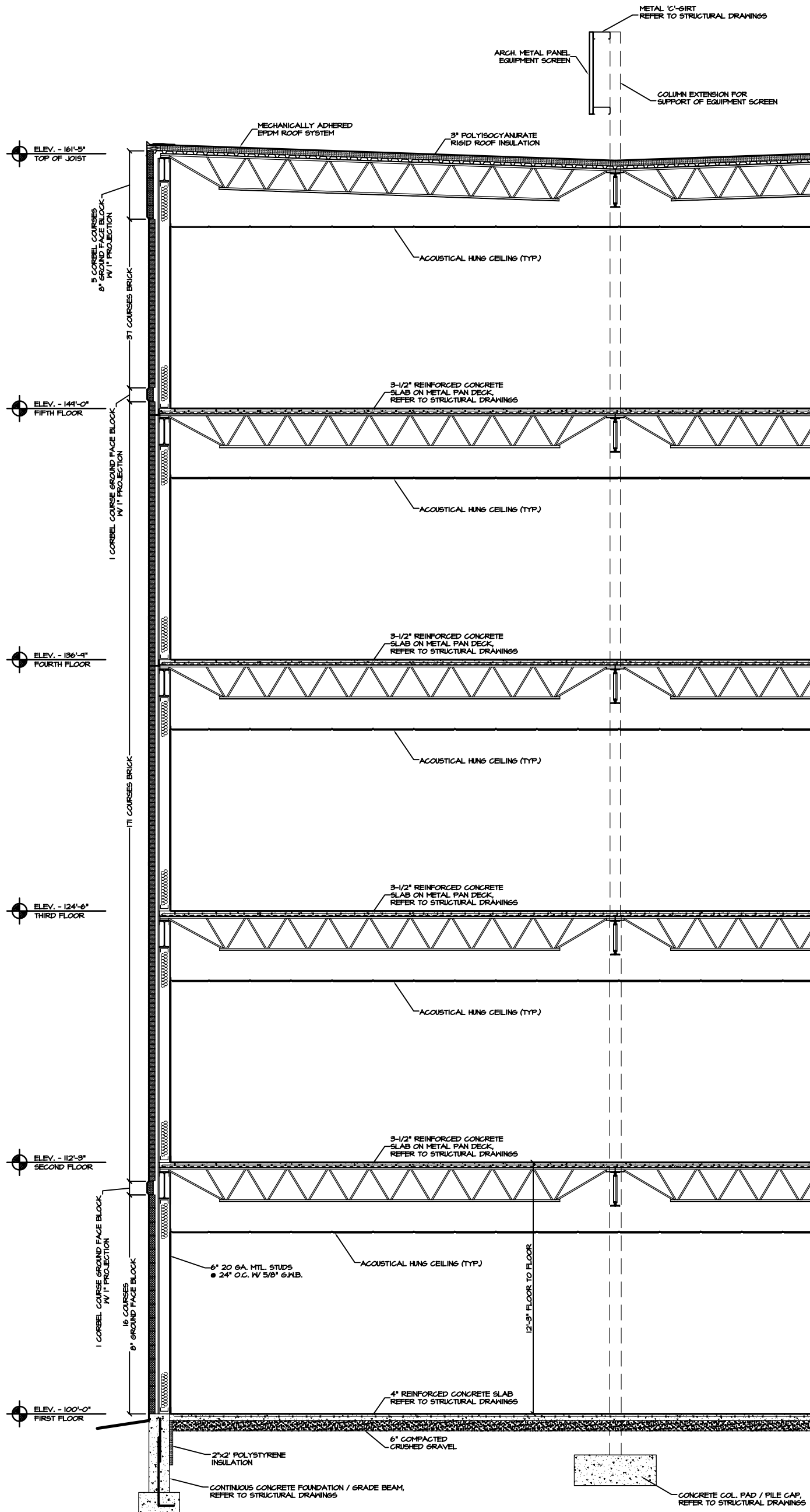
1 WALL SECTION A/C 5/8" = 1'-0"
