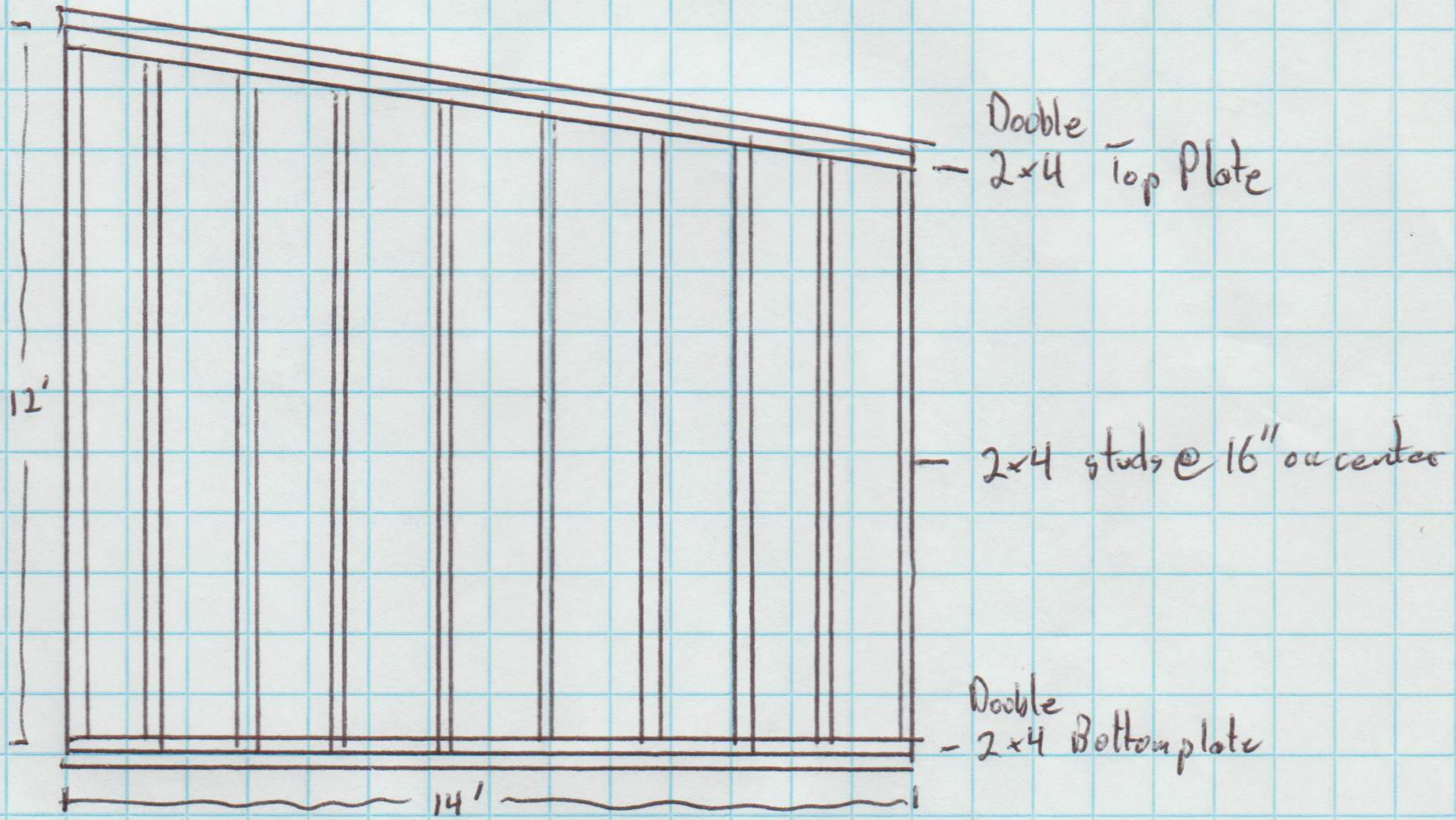
typical wall framing
