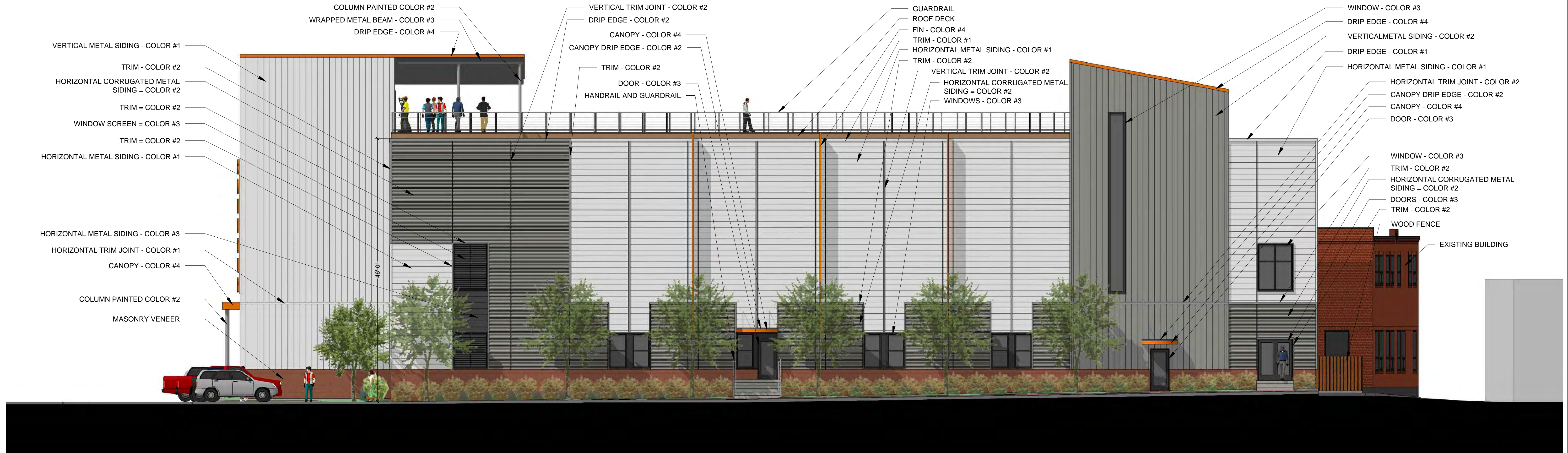
1 SOUTH ELEVATION 1/8" = 1'-0"
