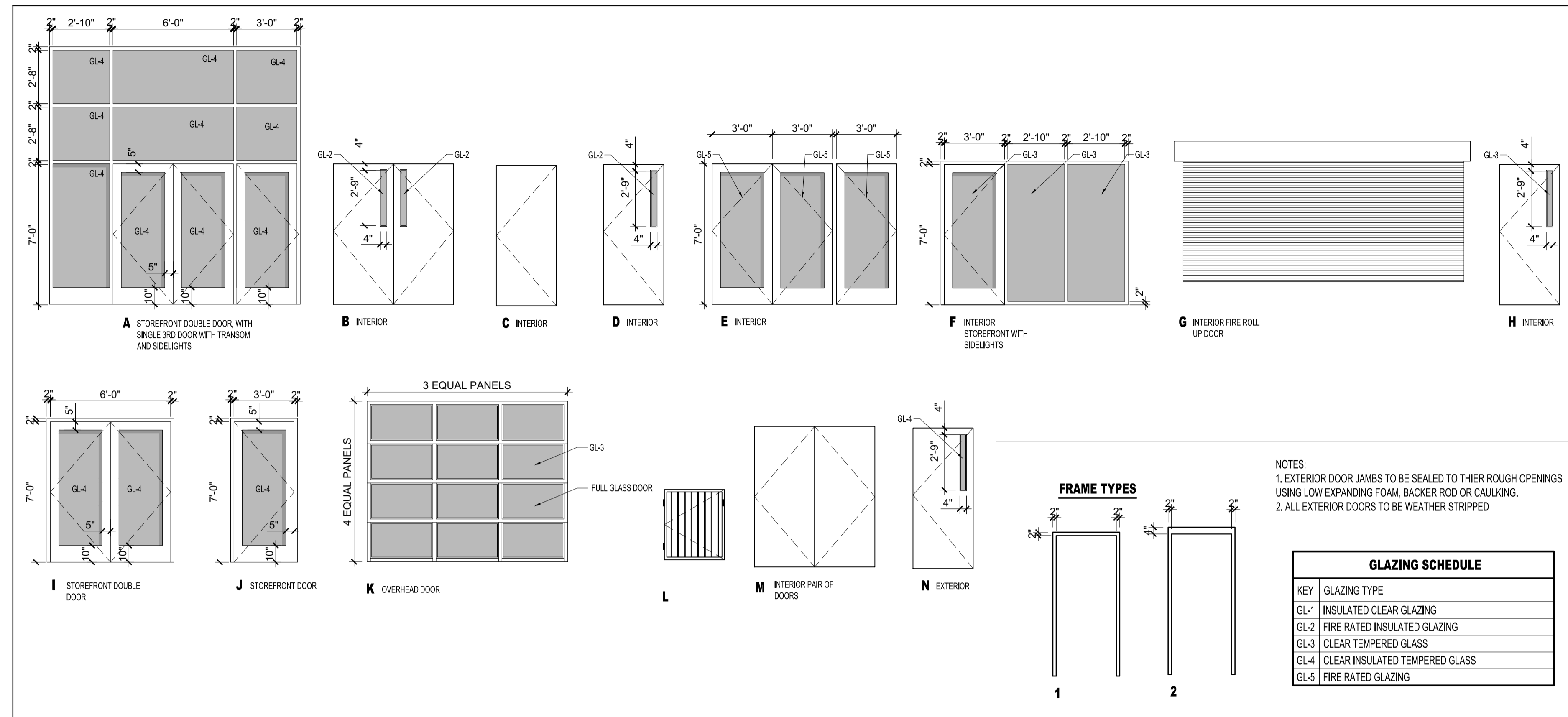
1 DOOR TYPES 1/4" = 1'-0"
