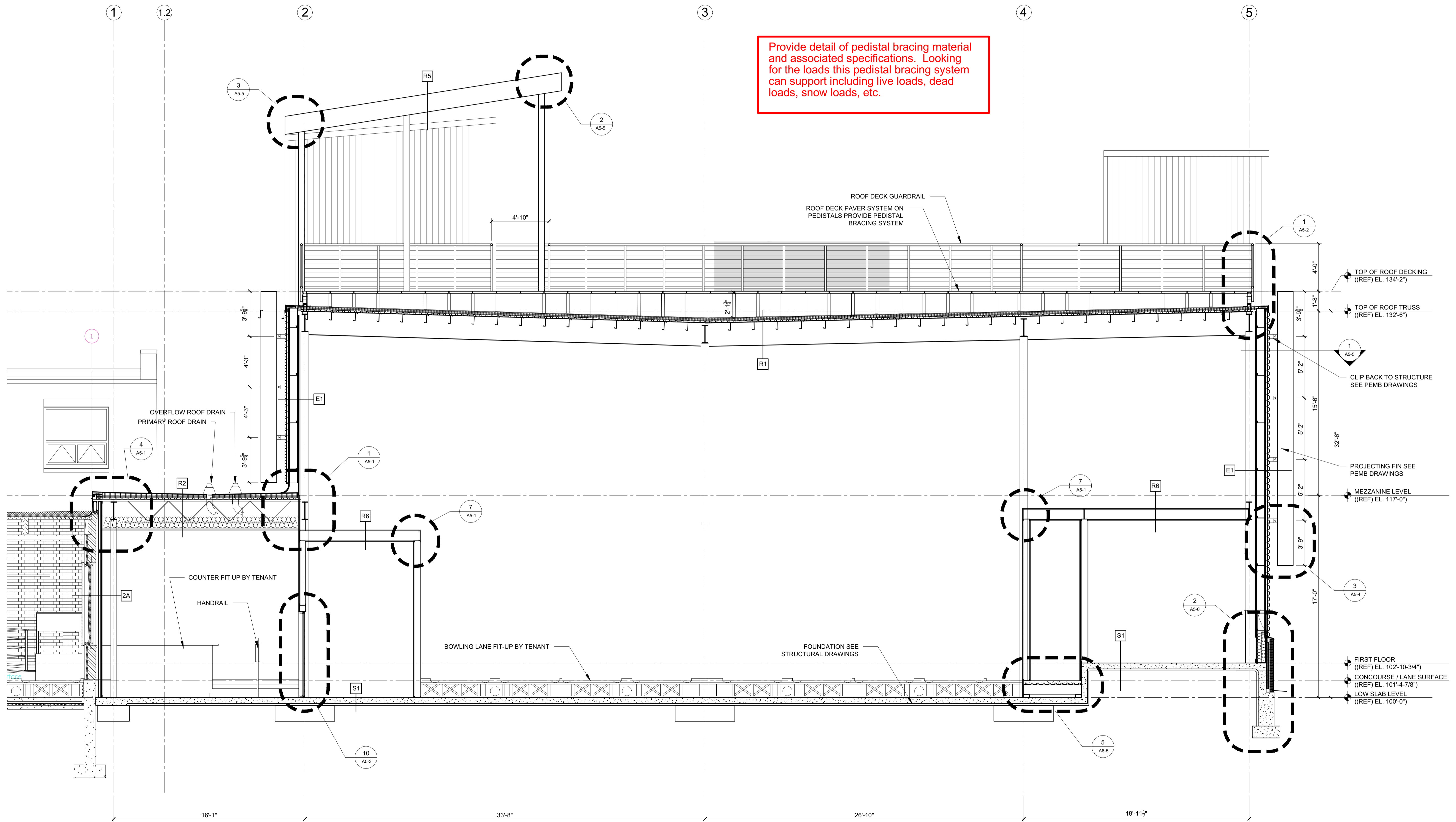
1 SECTION 1/4" = 1'-0"
