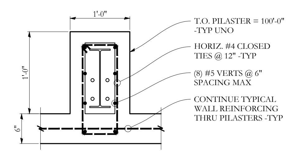
3/4"=1'-0 M DETAIL S2.2 TYPICAL STRAIGHT PILASTER
