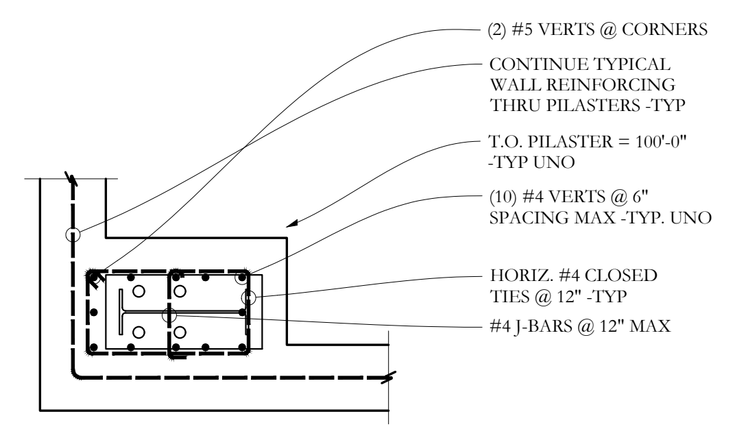
3/4"=1'-0 L DETAIL S2.2 TYPICAL CORNER PILASTER
