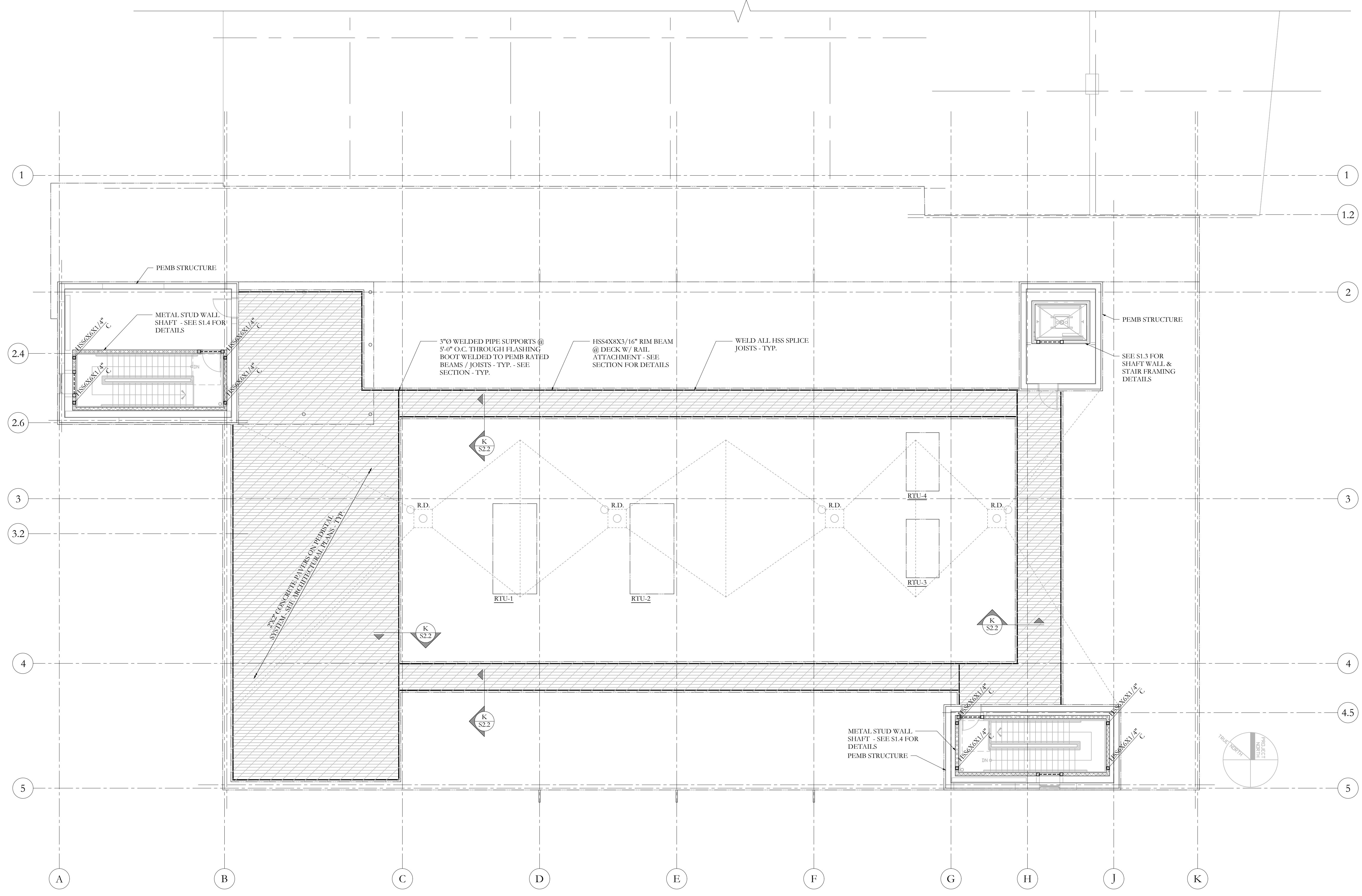
ROOF LEVEL PLAN SCALE 1/8"=1'-0" NOTES: 1. REFERENCE AND COORDINATE ALL DIMENSIONS W/ ARCHITECTURAL AND FRAMING PLANS - TYP.
