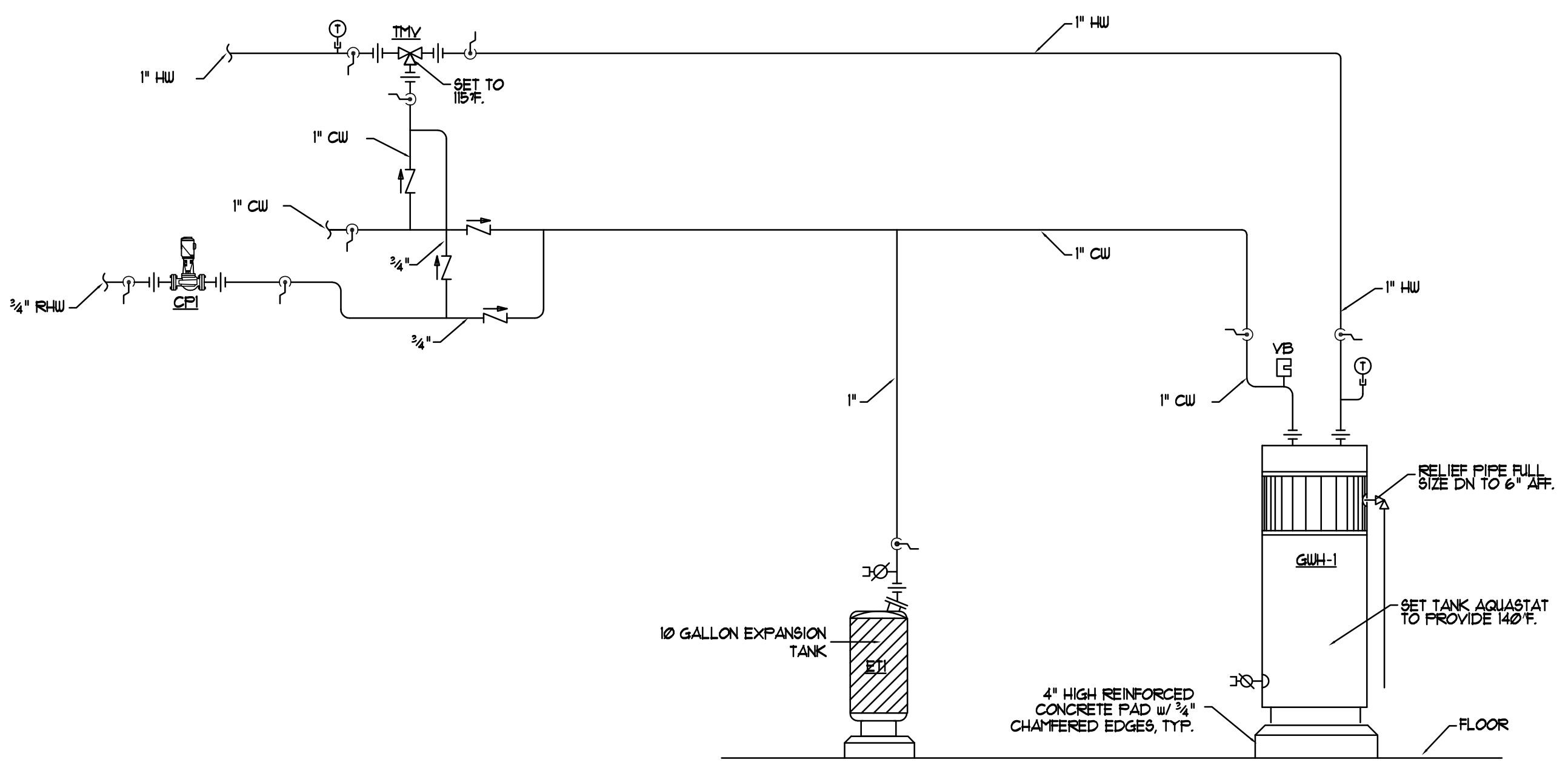
DOMESTIC HOT WATER PIPING SCHEMATIC NTS
