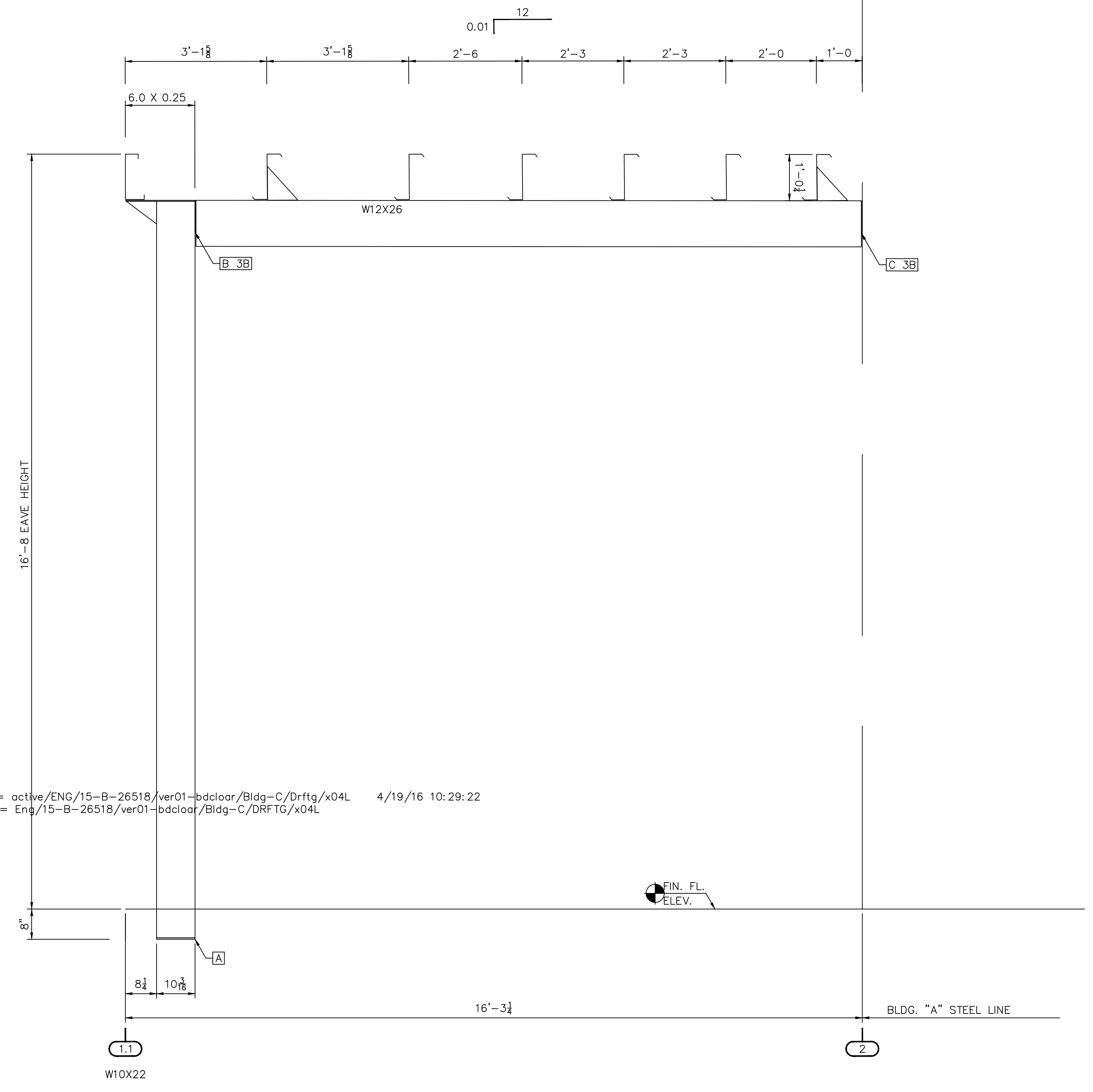
CROSS SECTION AT FRAME LINES "B-F"
