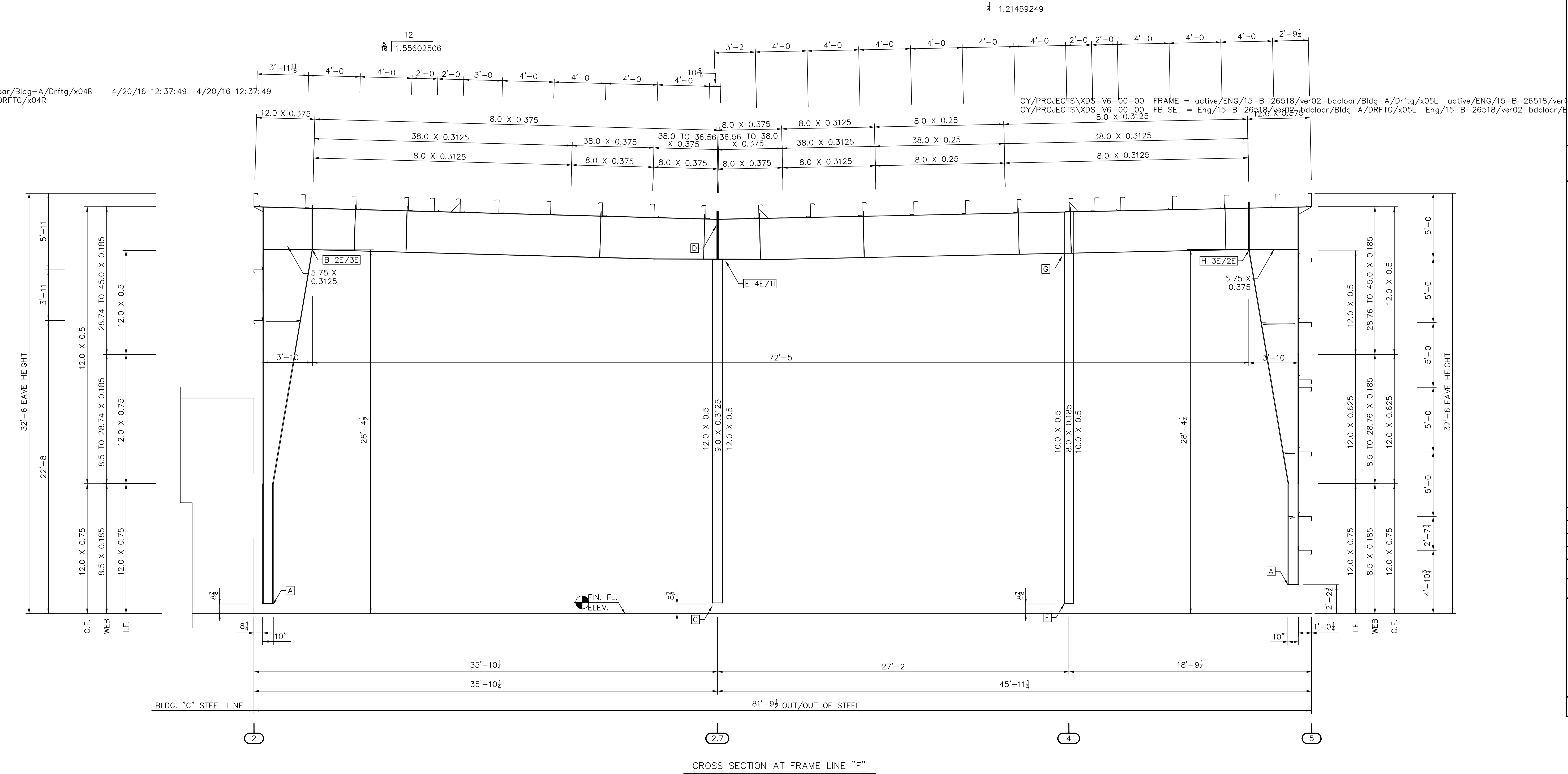
CROSS SECTION AT FRAME LINE "F"
