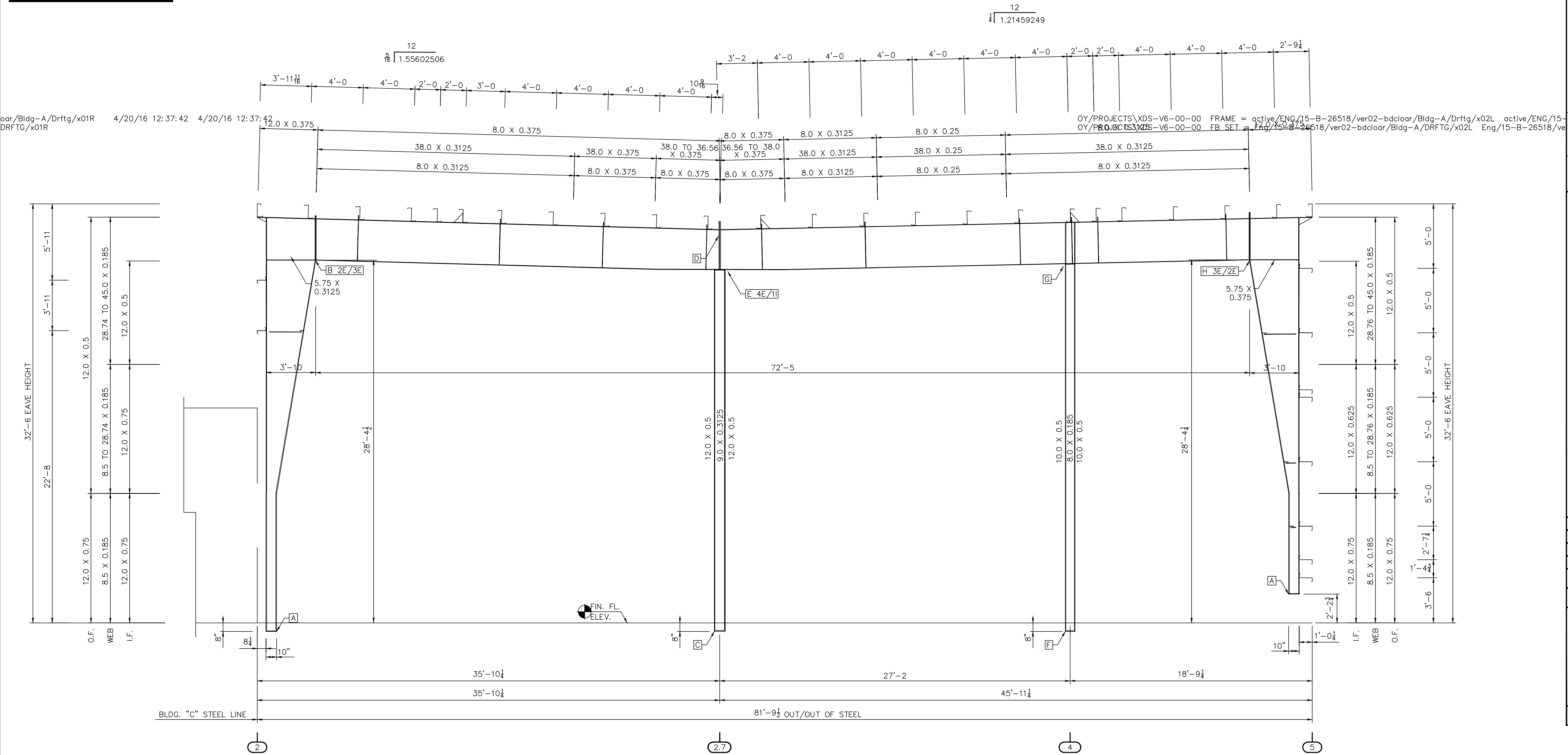
CROSS SECTION AT FRAME LINE "C"
