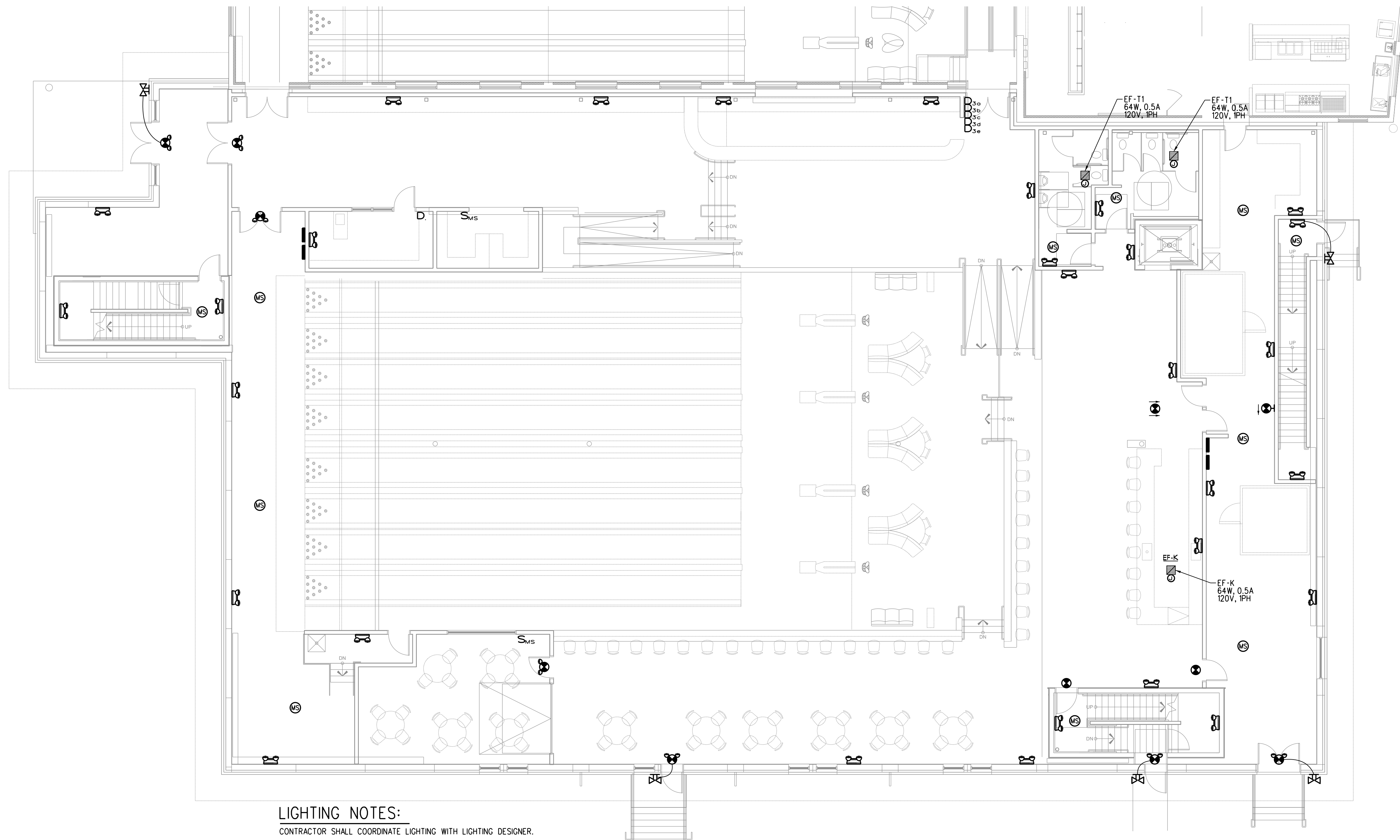
FIRST FLOOR LIGHTING PLAN SCALE: 1/8" = 1'-0"
