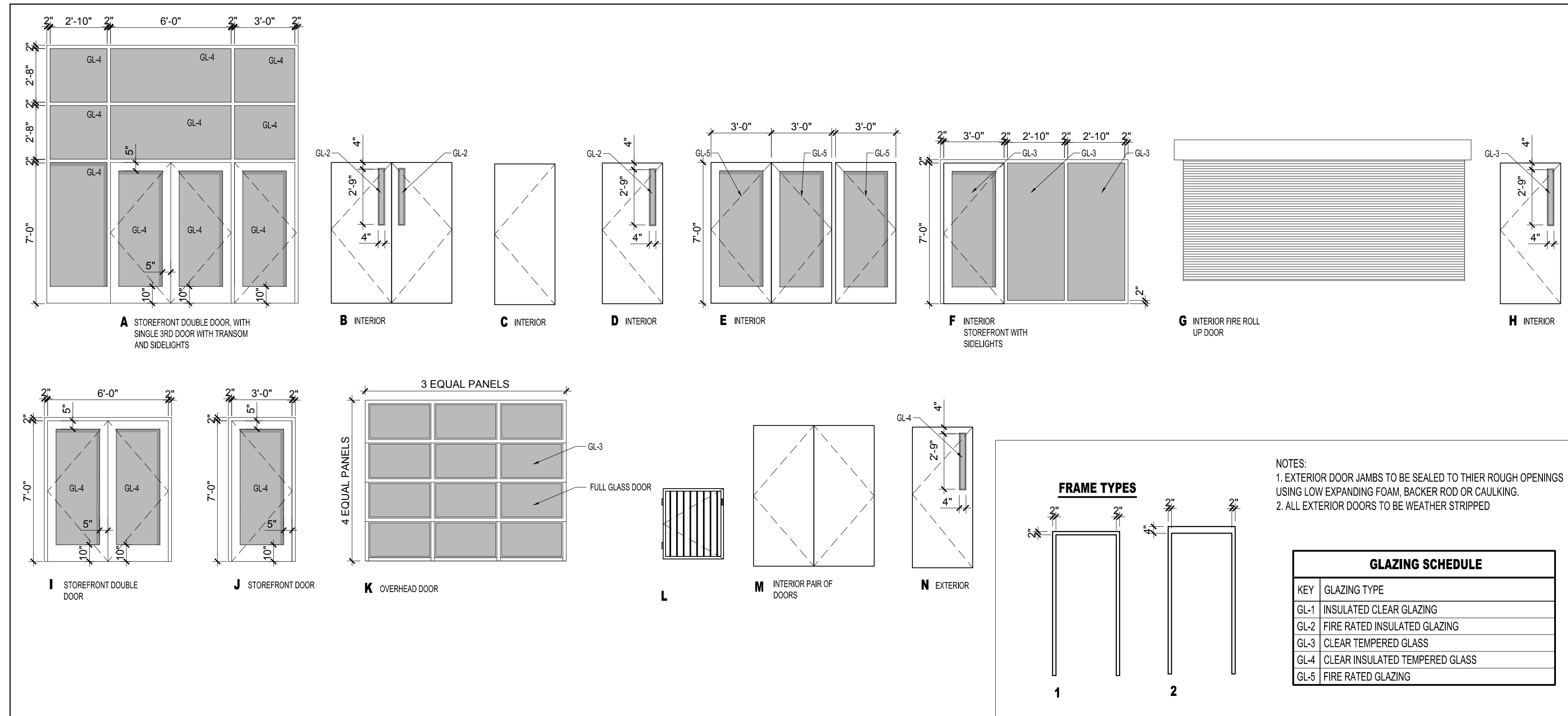
1 DOOR TYPES 1/4" = 1'-0"
