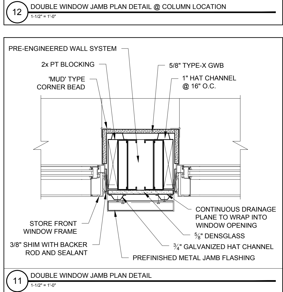
12 DOUBLE WINDOW JAMB PLAN DETAIL @ COLUMN LOCATION 1/12" = 1'-0"
