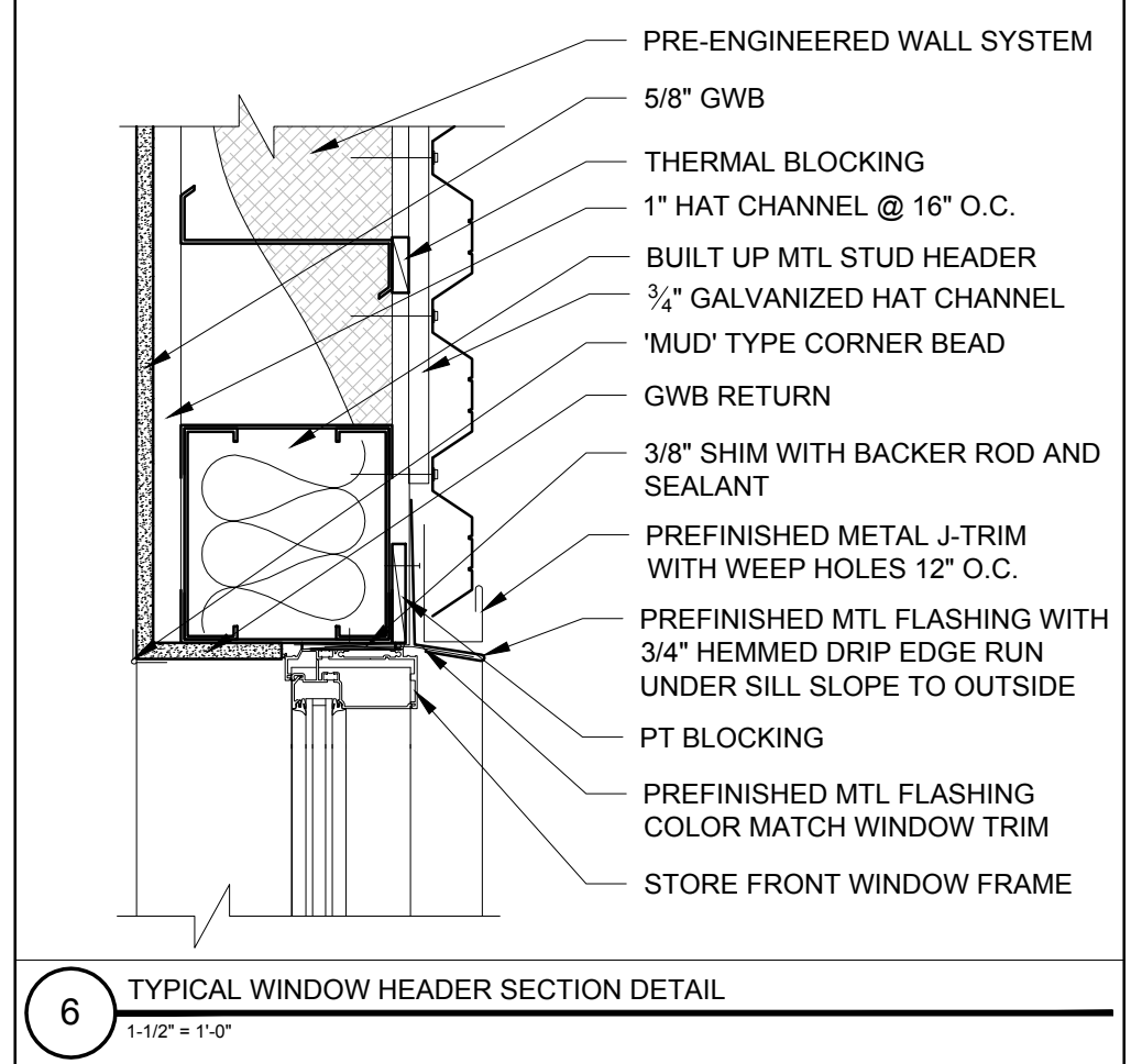
7 TYPICAL WINDOW PLAN DETAIL 1/12" = 1'-0"
