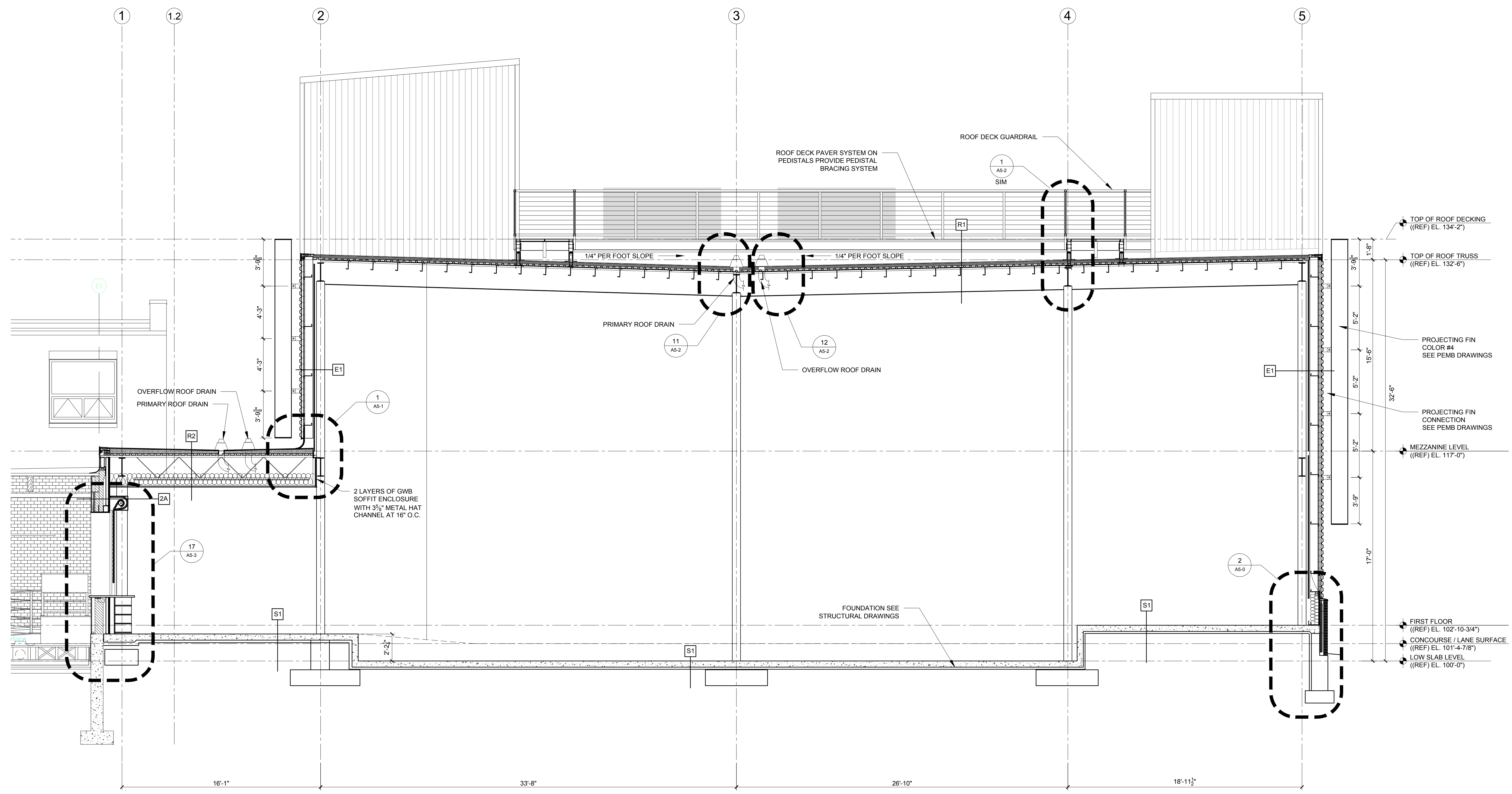
1 SECTION 3/4" = 1'-0"
