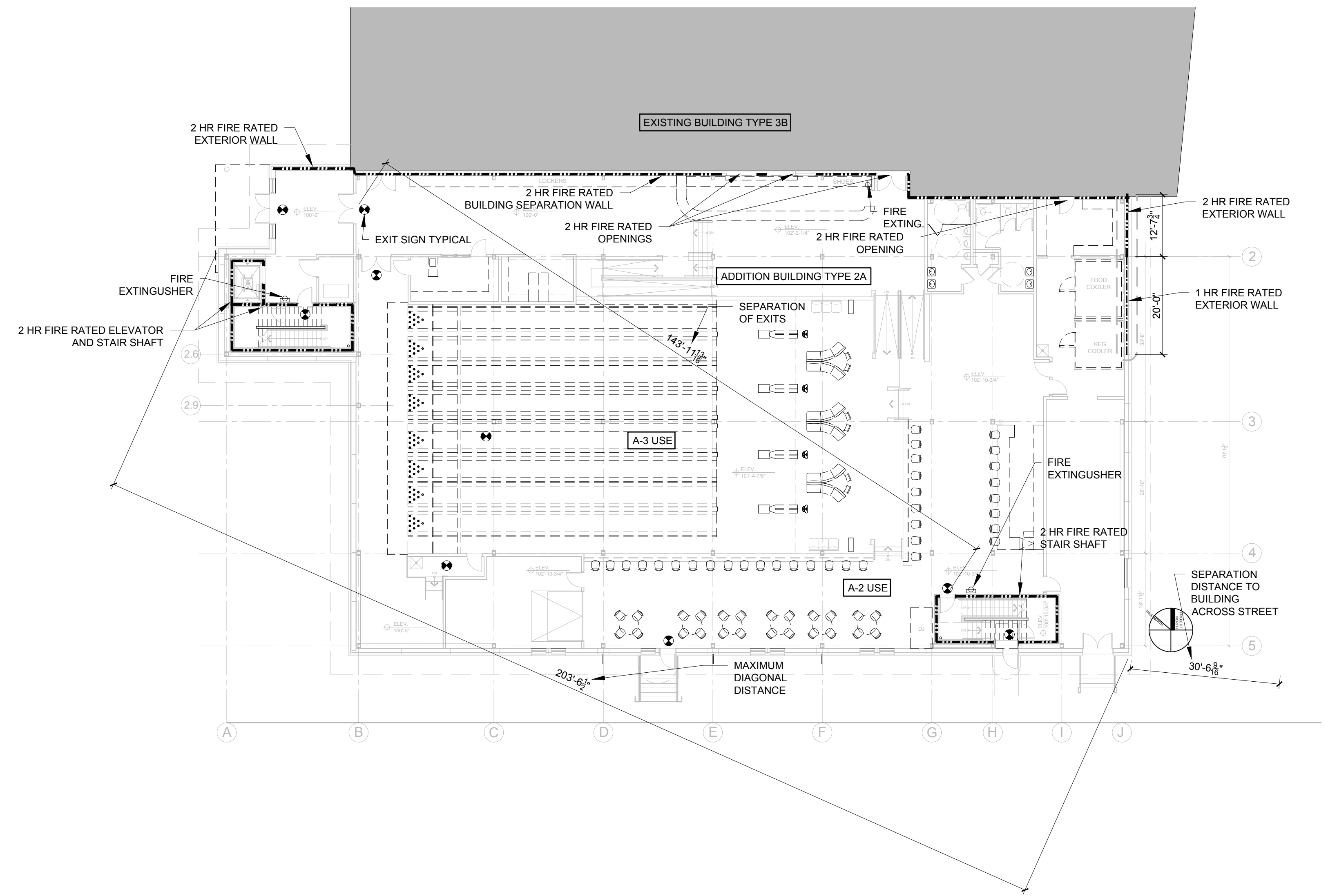
1 FIRST FLOOR CODE REVIEW PLAN 1/16" = 1'-0"
