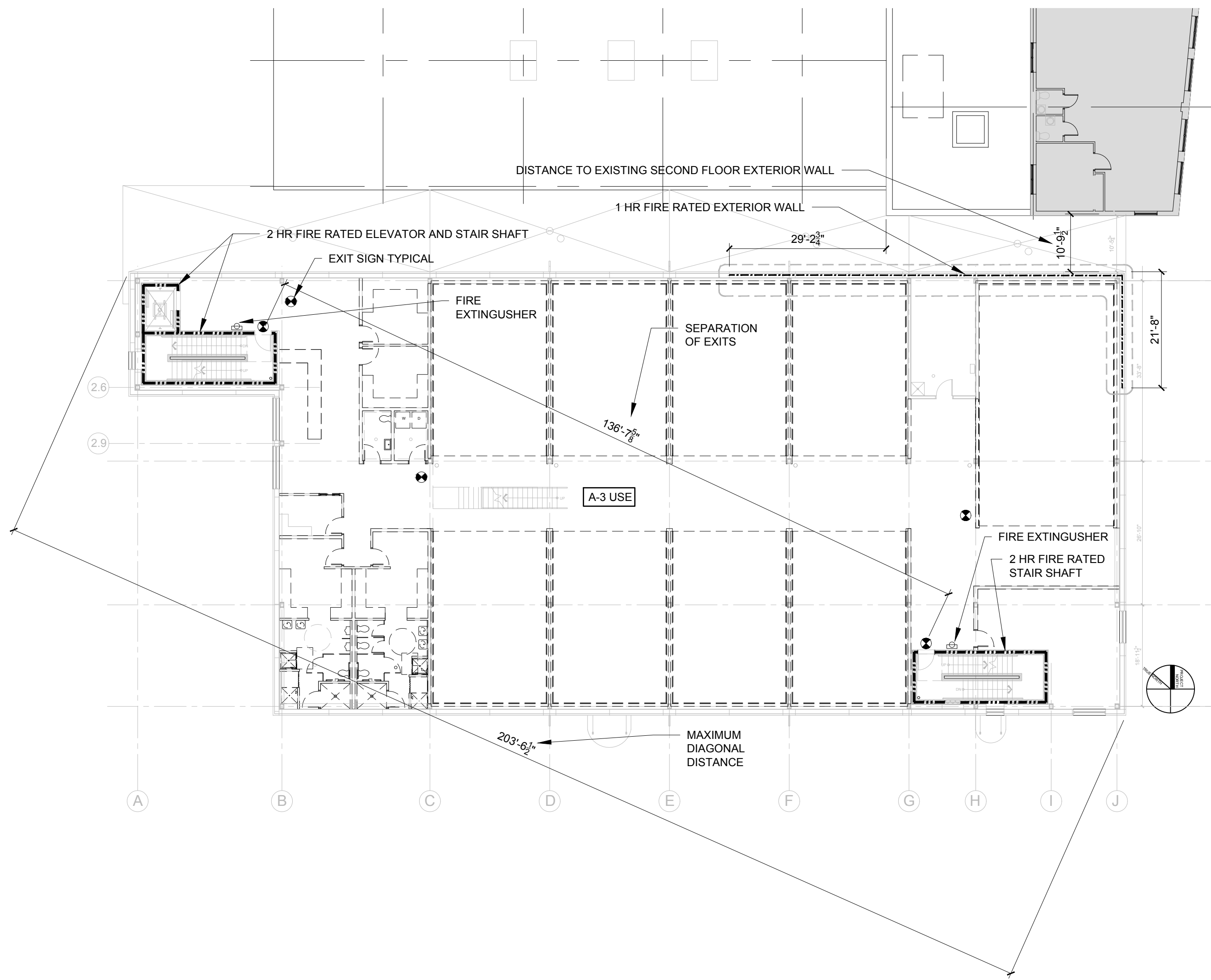
2 SECOND FLOOR CODE REVIEW PLAN 1/16" = 1'-0"
