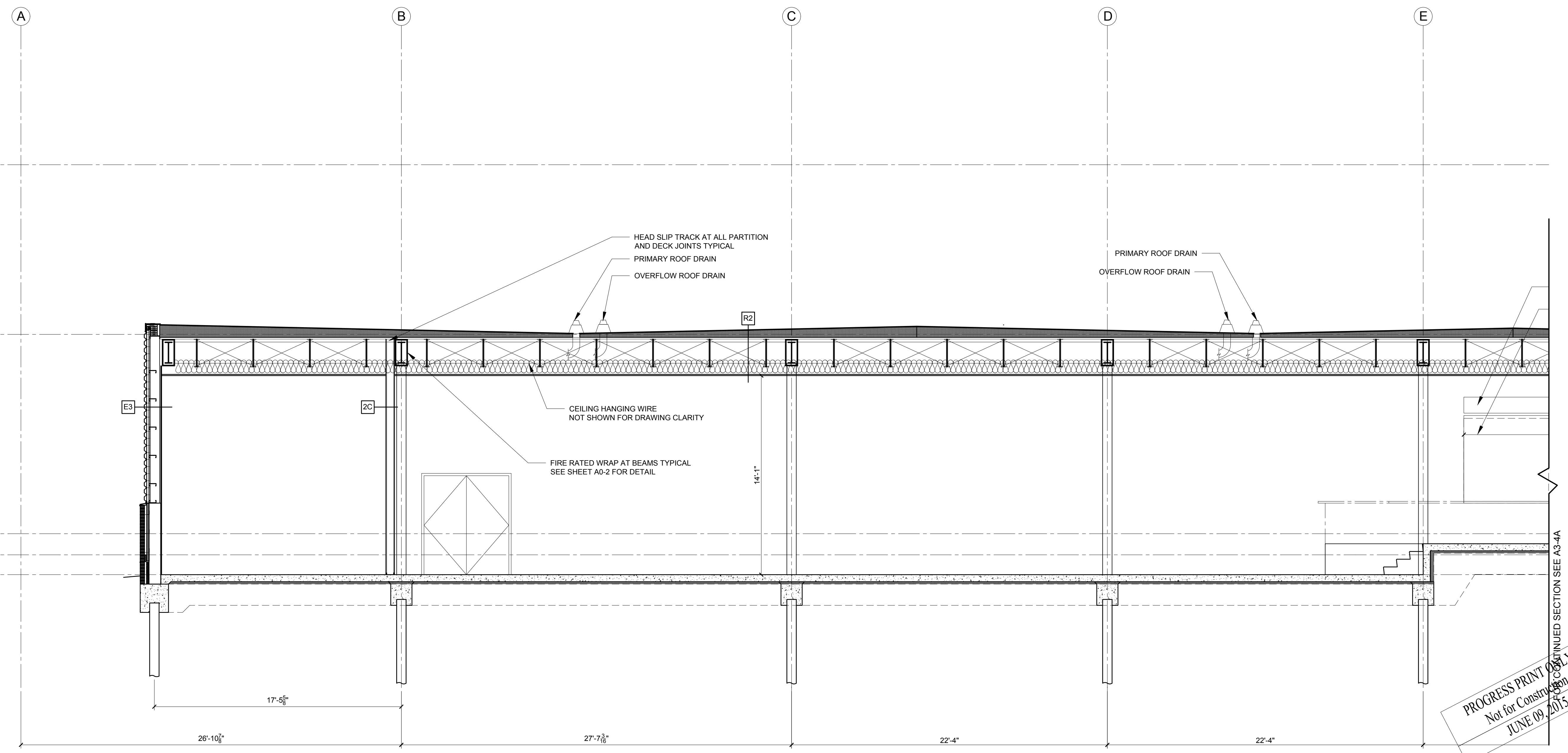
1 SECTION 1/4" = 1'-0"
