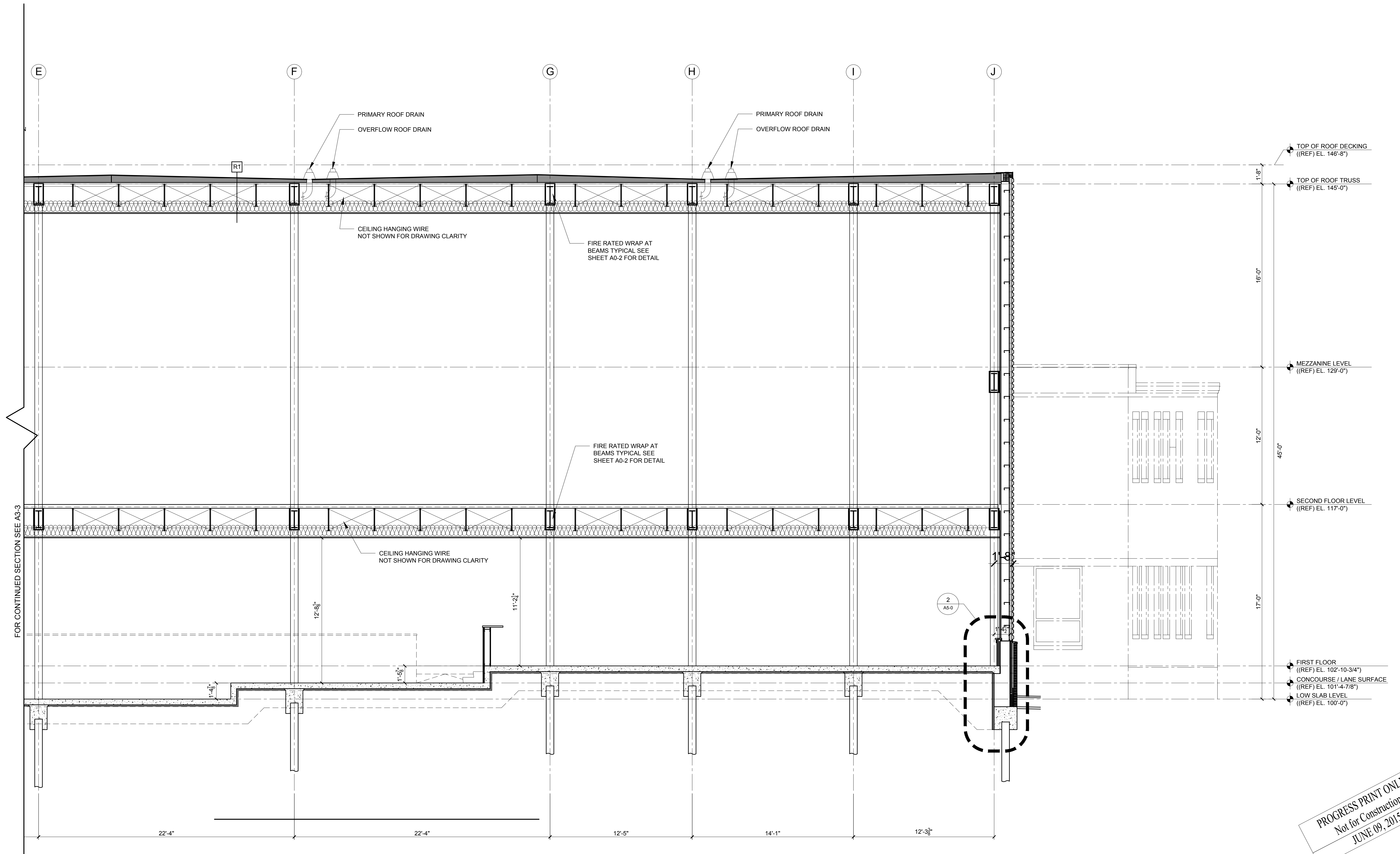
1 SECTION 1/4" = 1'-0"
