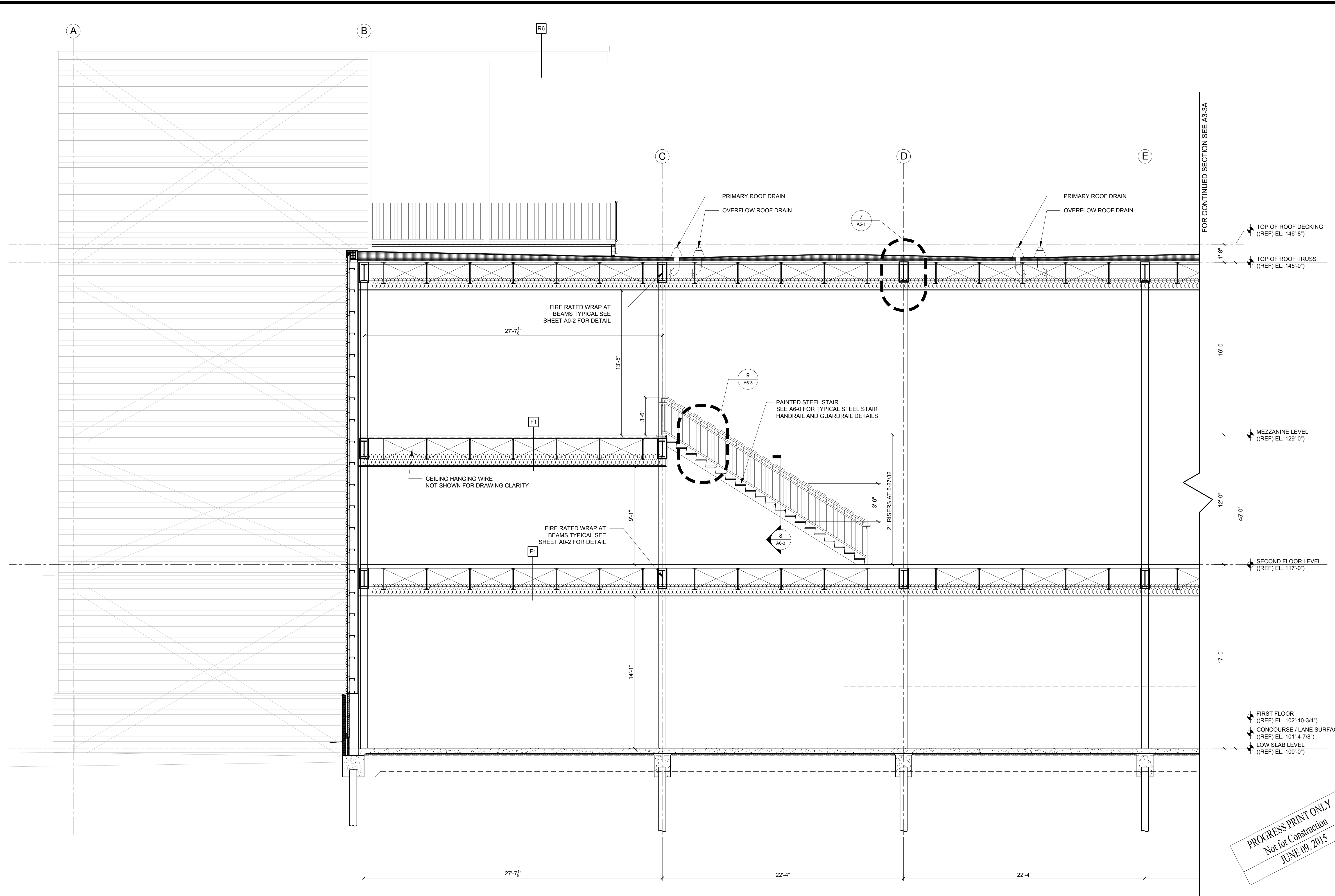
1 SECTION 1/4" = 1'-0"
