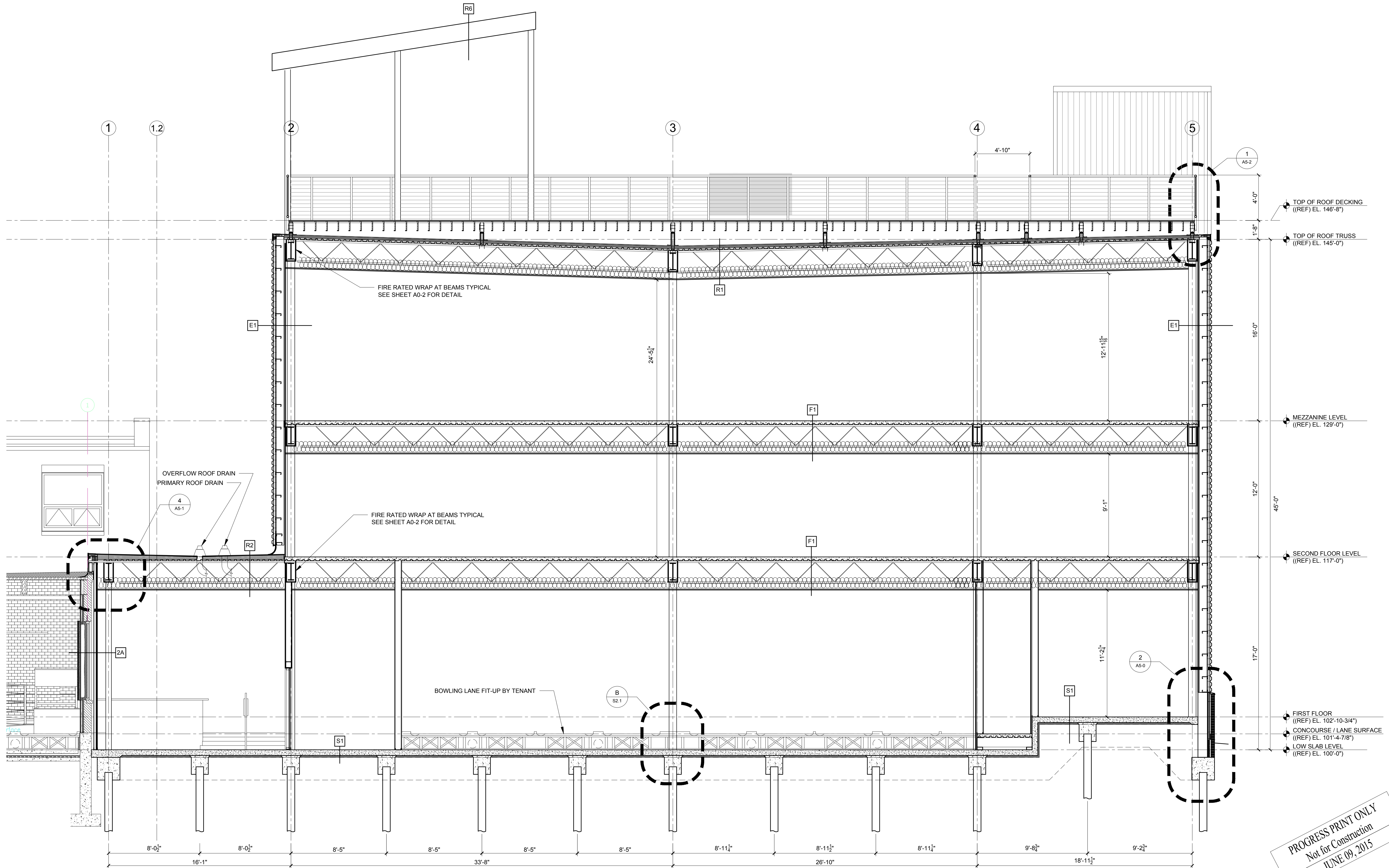
1 SECTION 1/4" = 1'-0"
