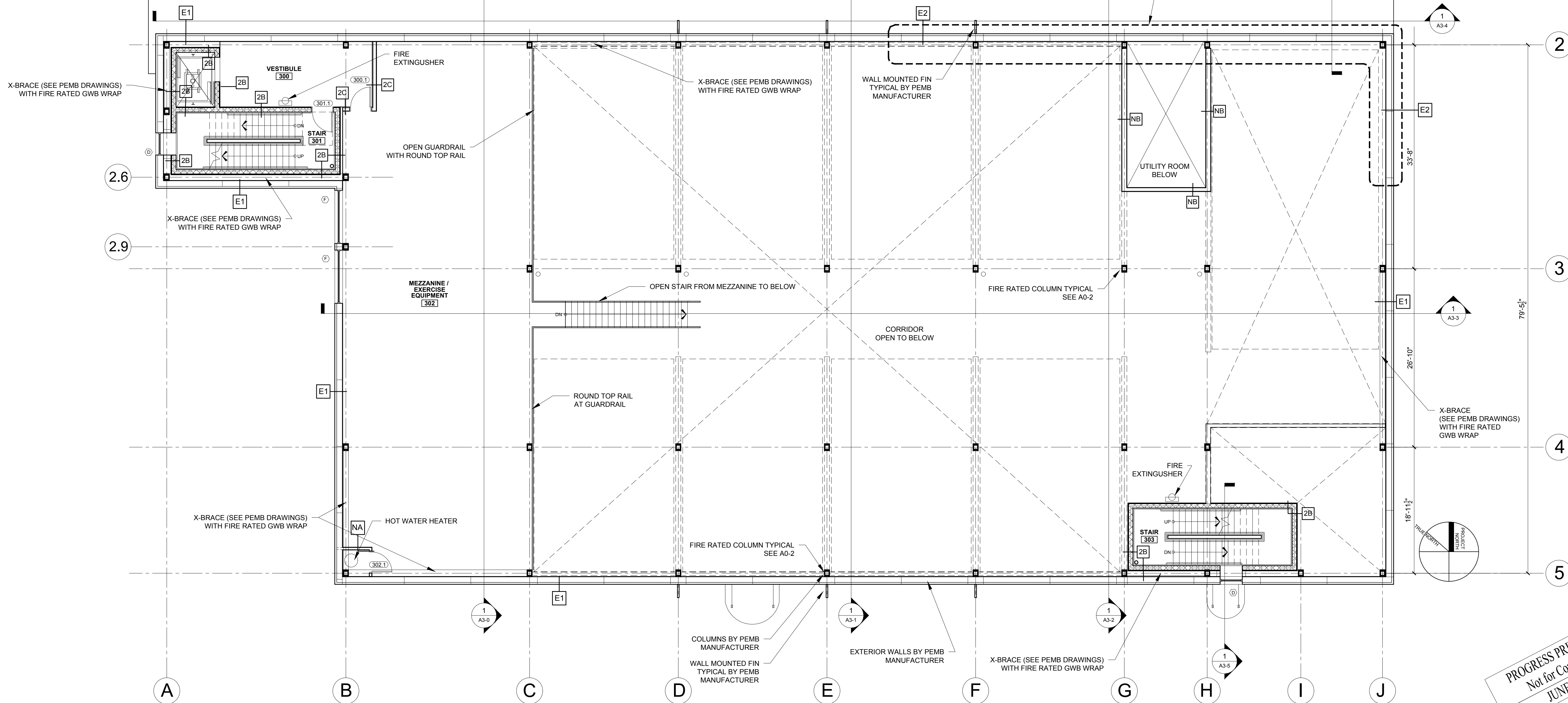
1 MEZZANINE LEVEL PLAN 1/8" = 1'-0"
