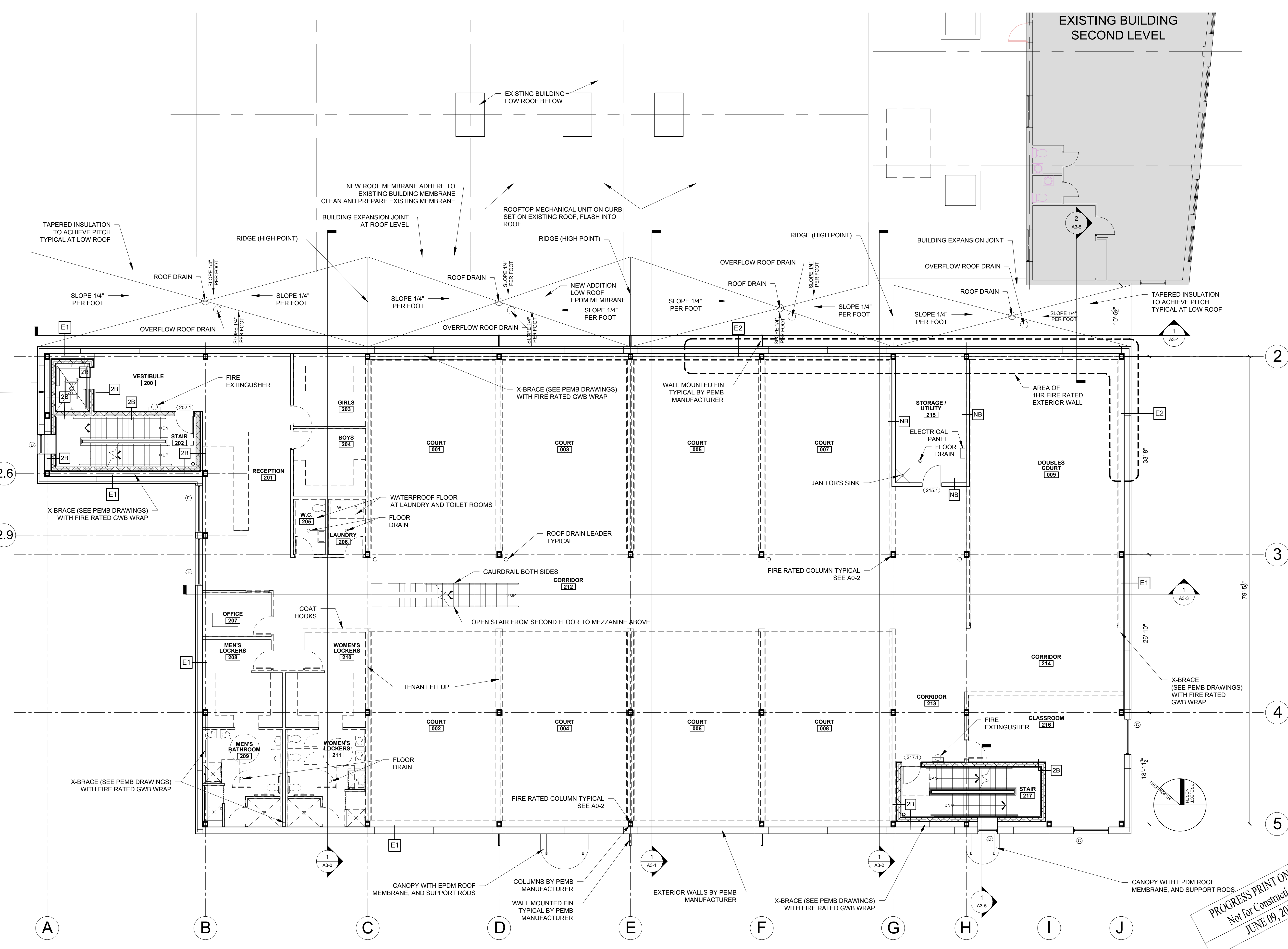
1 SECOND FLOOR PLAN 1/8" = 1'-0"
