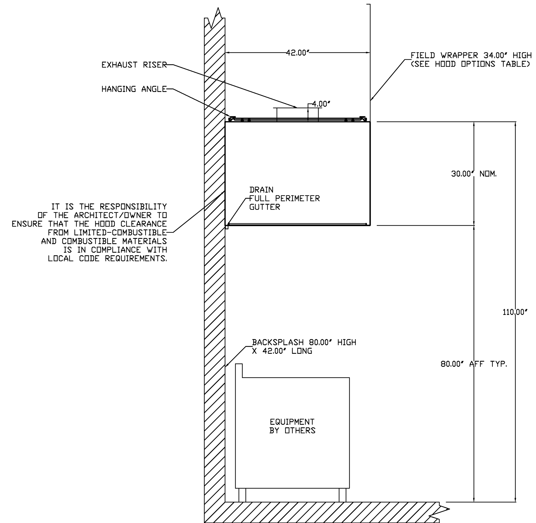
SECTION VIEW - MODEL 4230VHB-G
