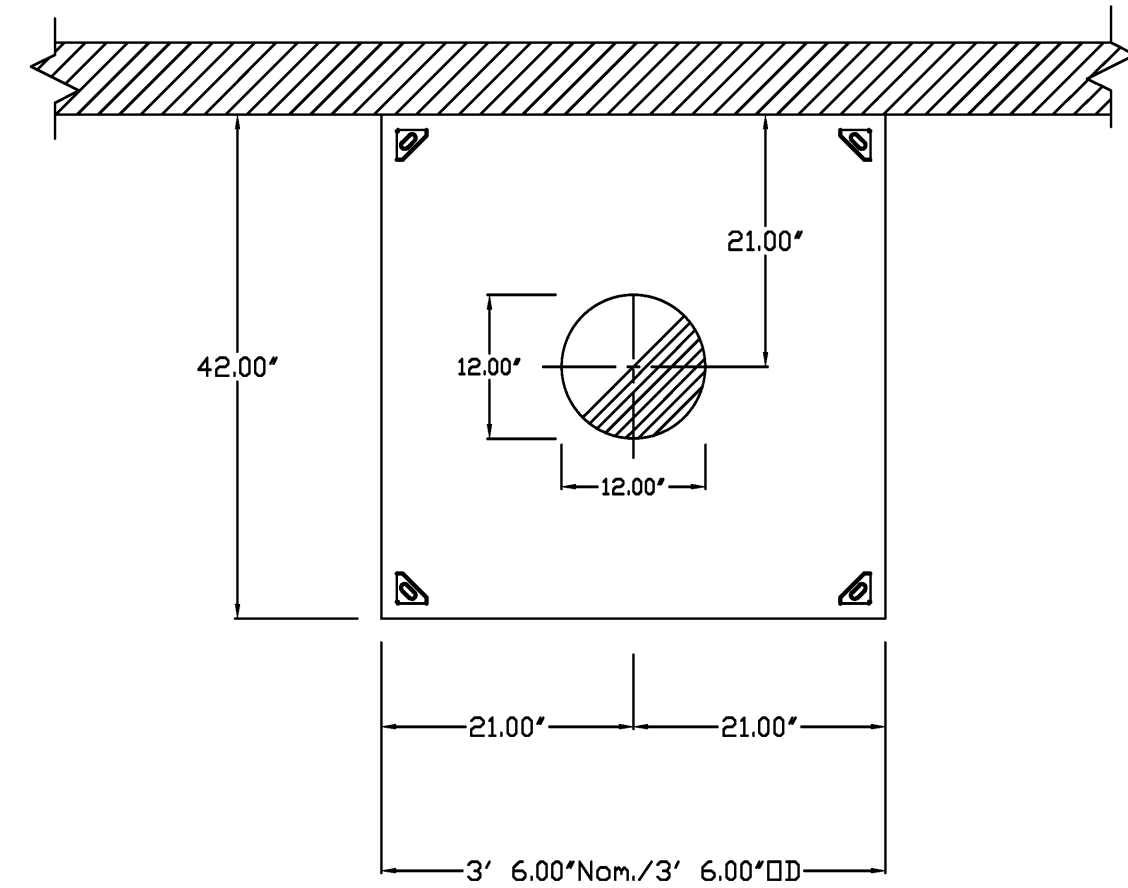
PLAN VIEW - Hood #2 (Dish) 3' 6.00" LONG 4230VHB-G
