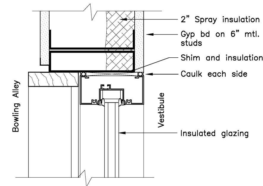
13 Storefront Head Detail - Alternate #3 Scale: 3" = 1'-0"
