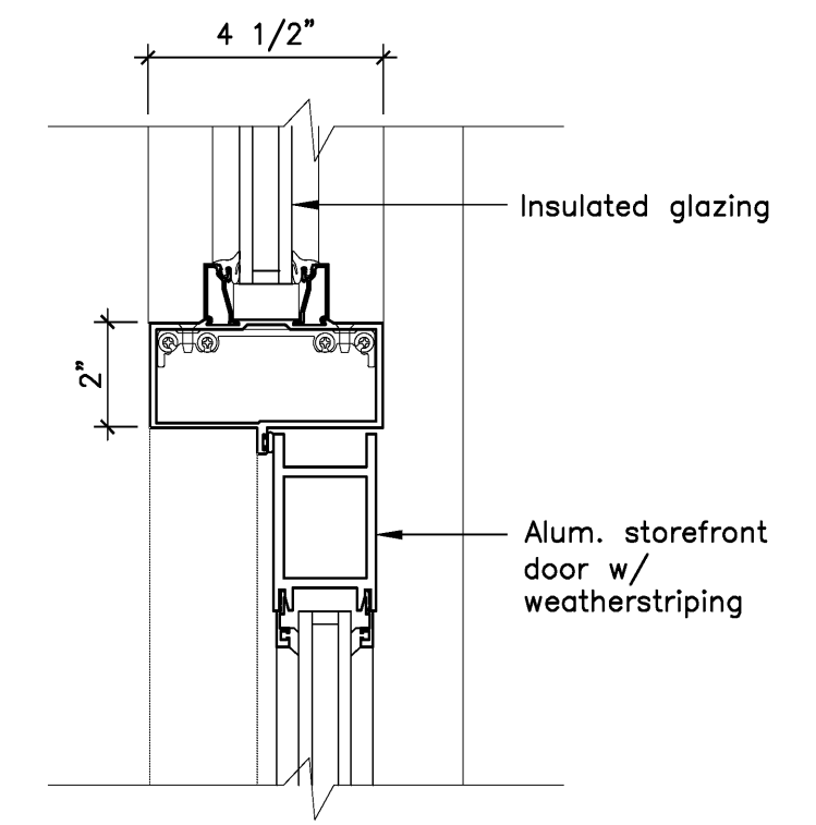
2 Storefront Door Head Detail Scale: 3" = 1'-0"
