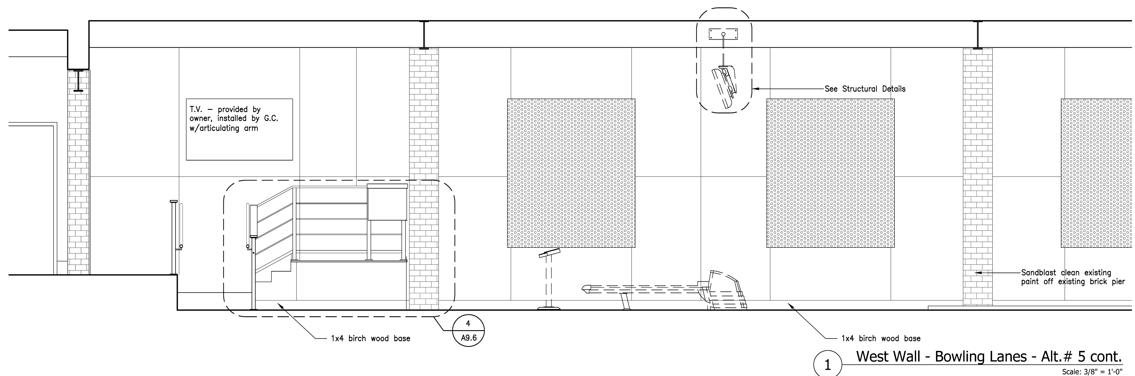
1 West Wall - Bowling Lanes - Alt. # 5 Scale: 3/8" = 1'-0"
