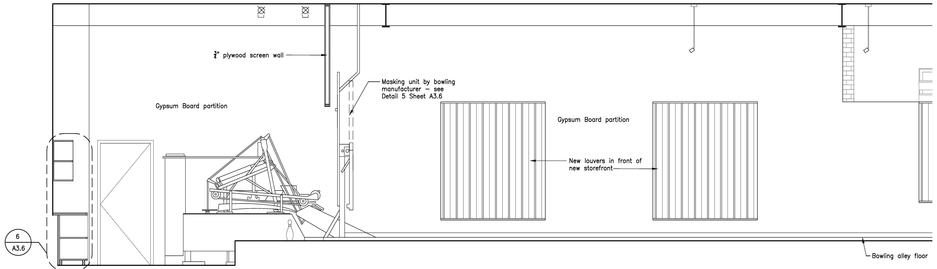
1 East Wall - Bowling Lanes & Pinsetter - Alt. # 4 cont. Scale: 3/8" = 1'-0"
