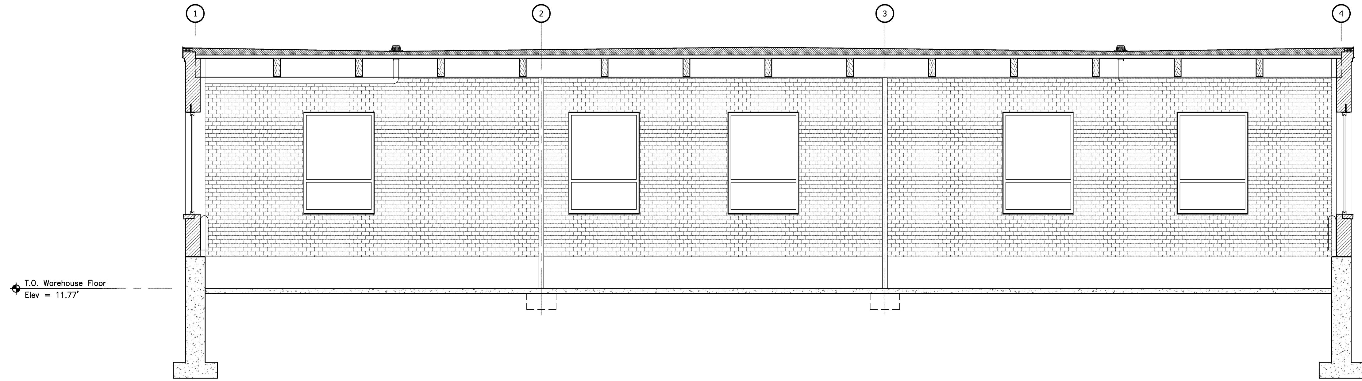
4 Existing Building Section Scale: 1/4" = 1'-0"
