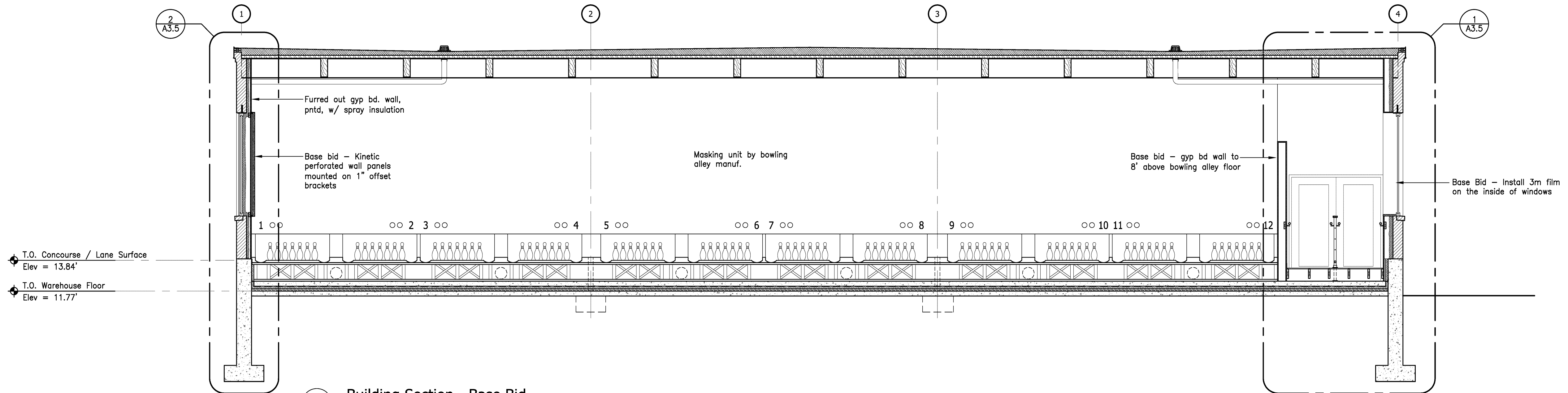
5 Building Section - Base Bid Scale: 1/4" = 1'-0"
