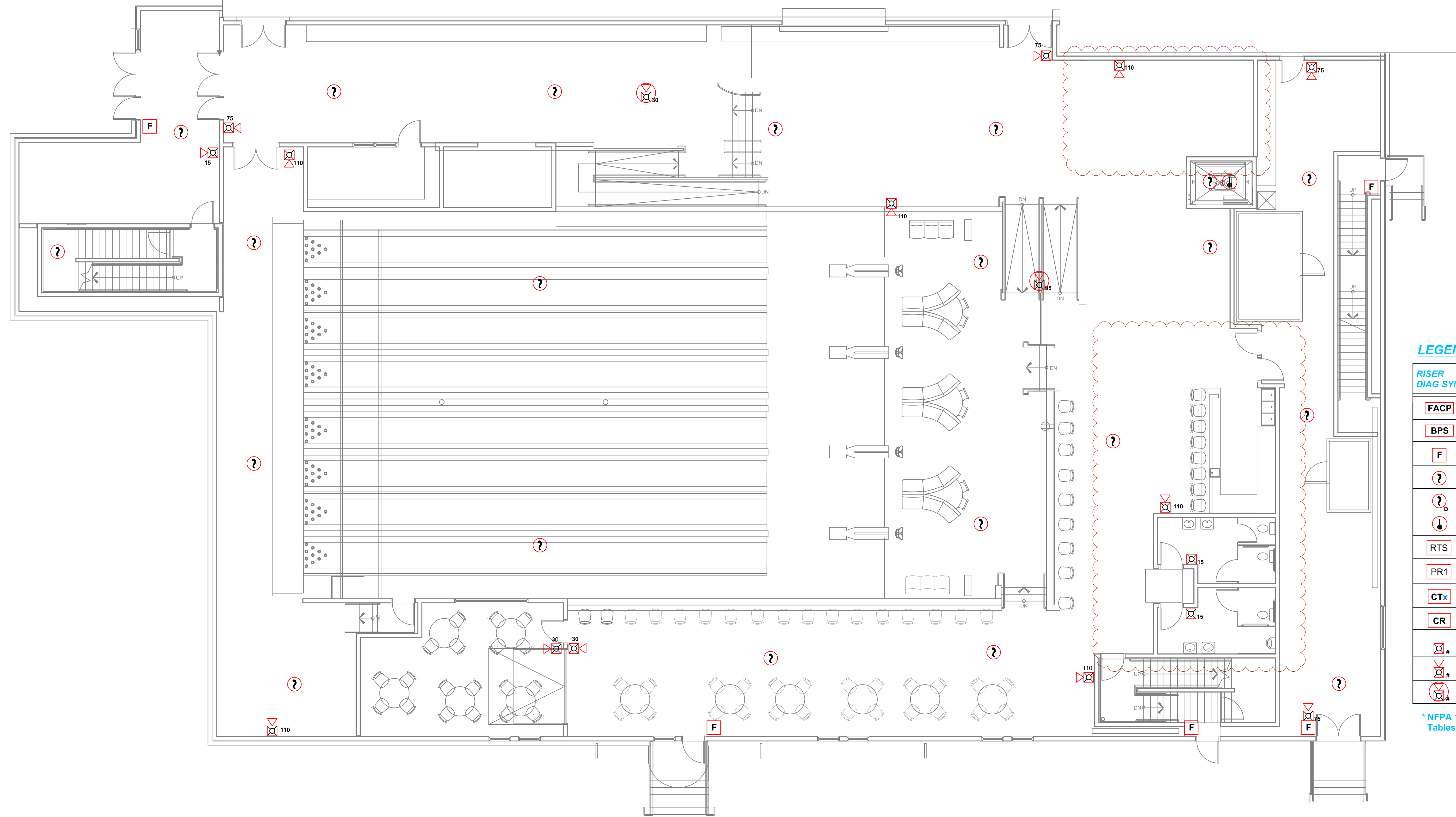
FIRST FLOOR POWER PLAN SCALE: 1/8" = 1'-0"
