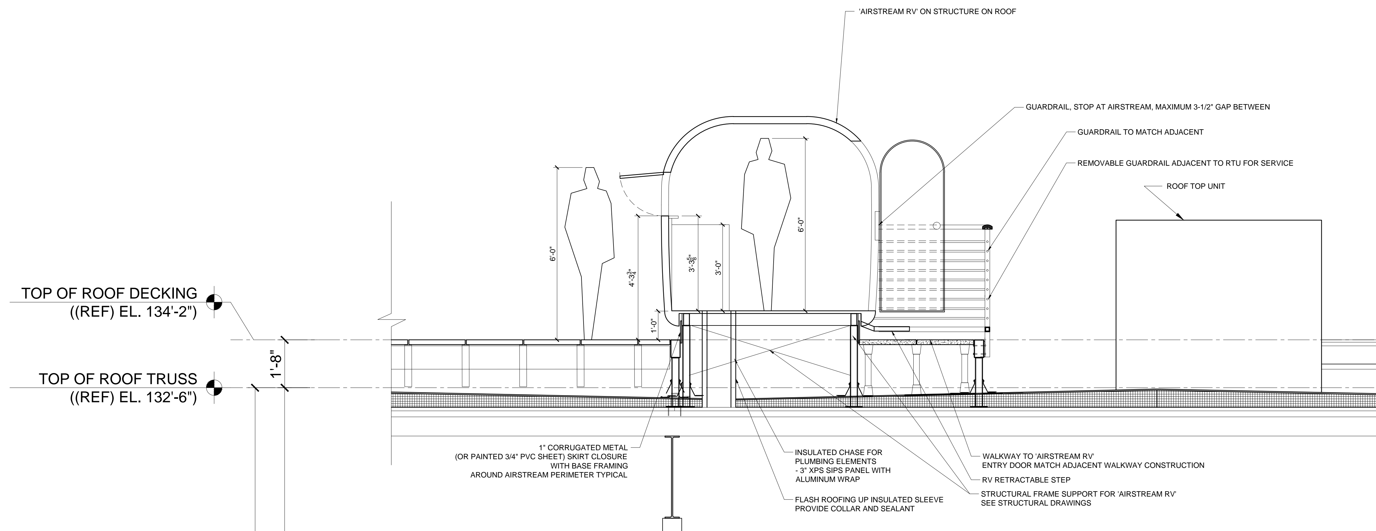
1 SECTION THROUGH AIRSTREAM RV AND DECK 1/2" = 1'-0"
