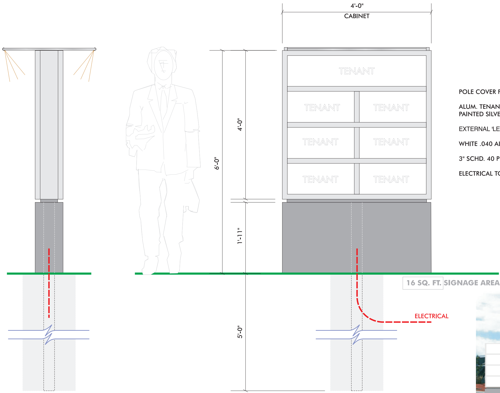
DOUBLE FACE EXTERNALLY ILLUMINATED TENANT PYLON SCALE: 3/4"=1'-0" (2) SIGNS REQUIRED
