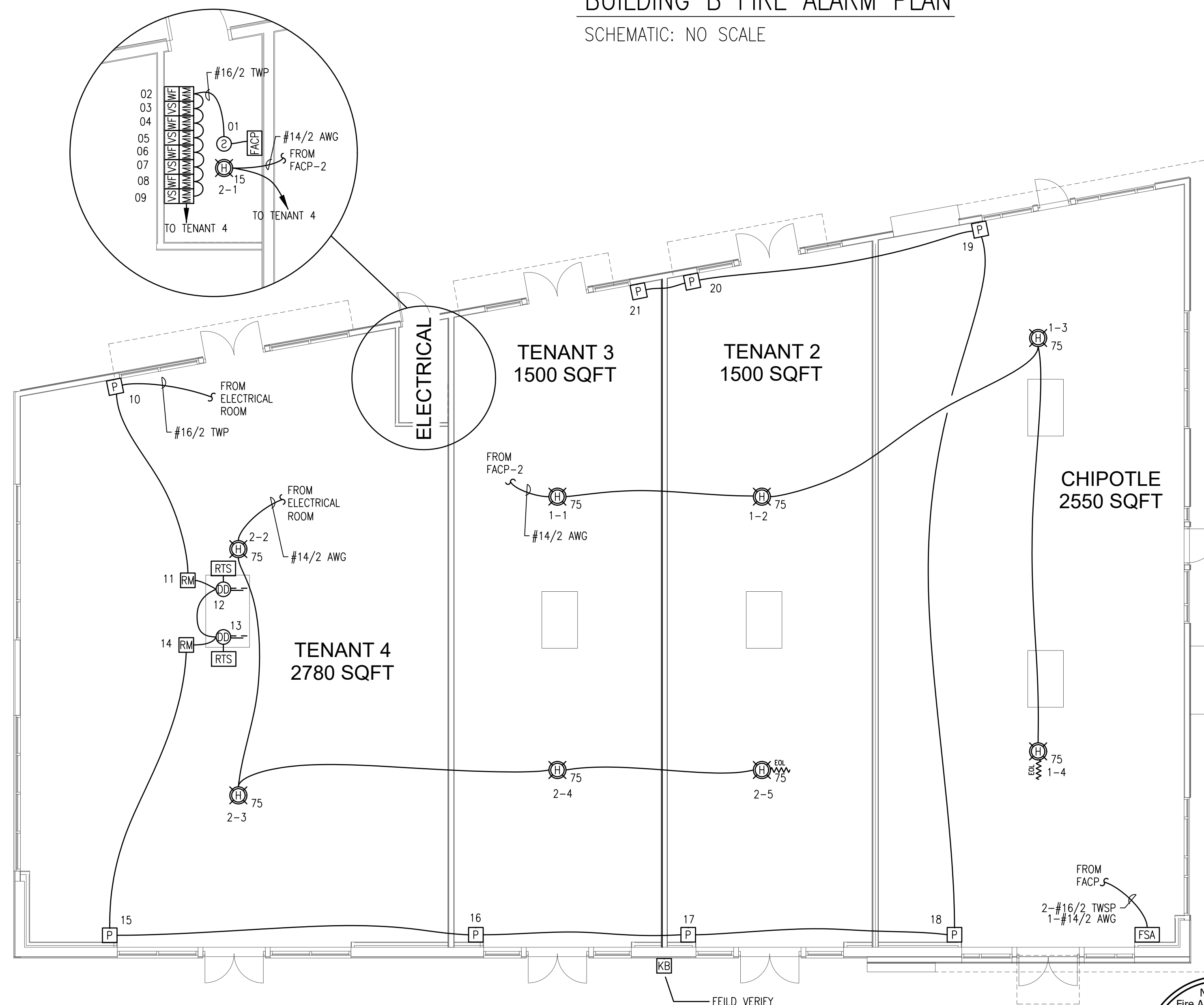
BUILDING B FIRE ALARM PLAN SCALE: 1/8"=1'-0"
