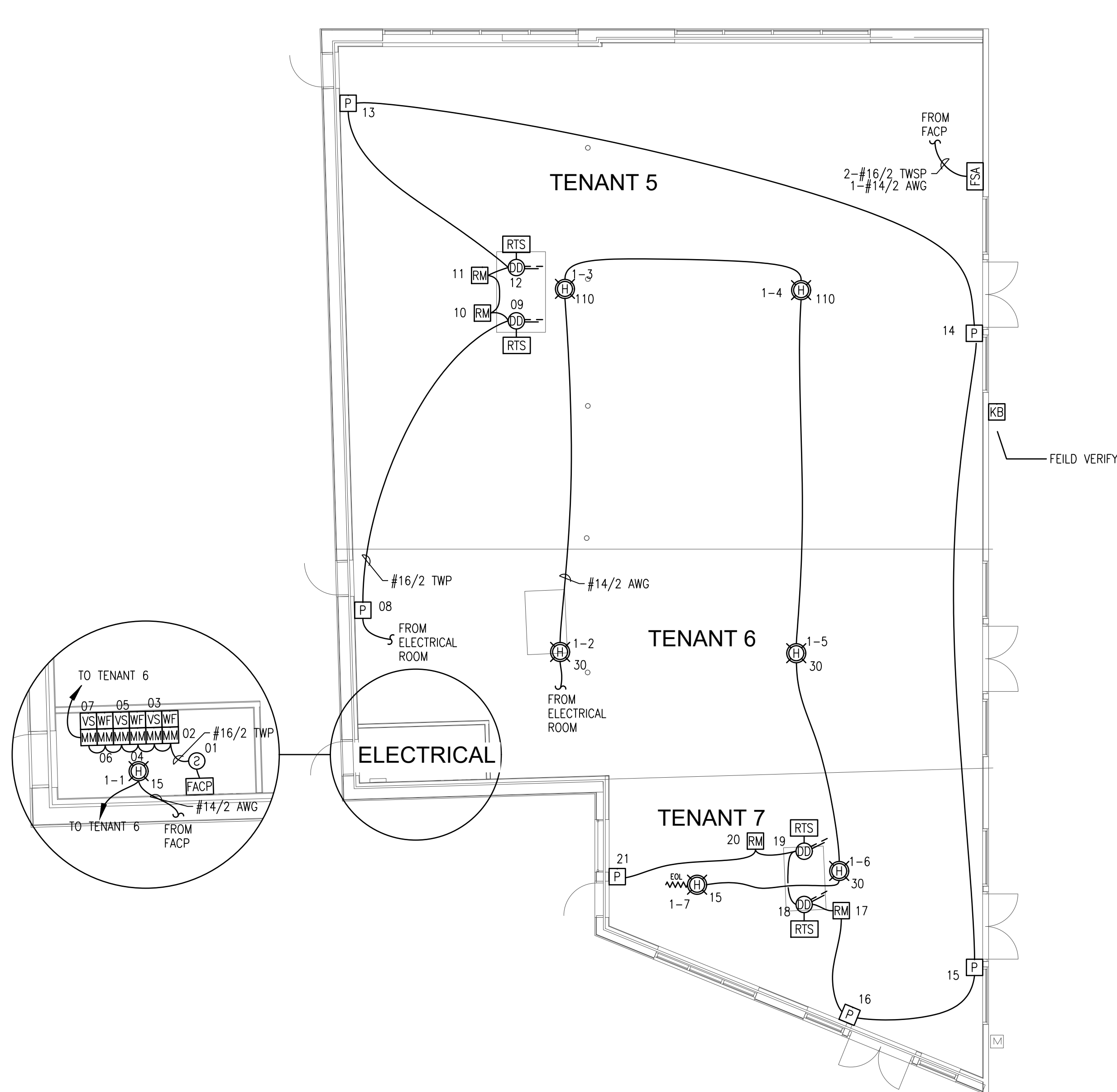
BUILDING A FIRE ALARM PLAN SCALE: 1/8"=1'-0"
