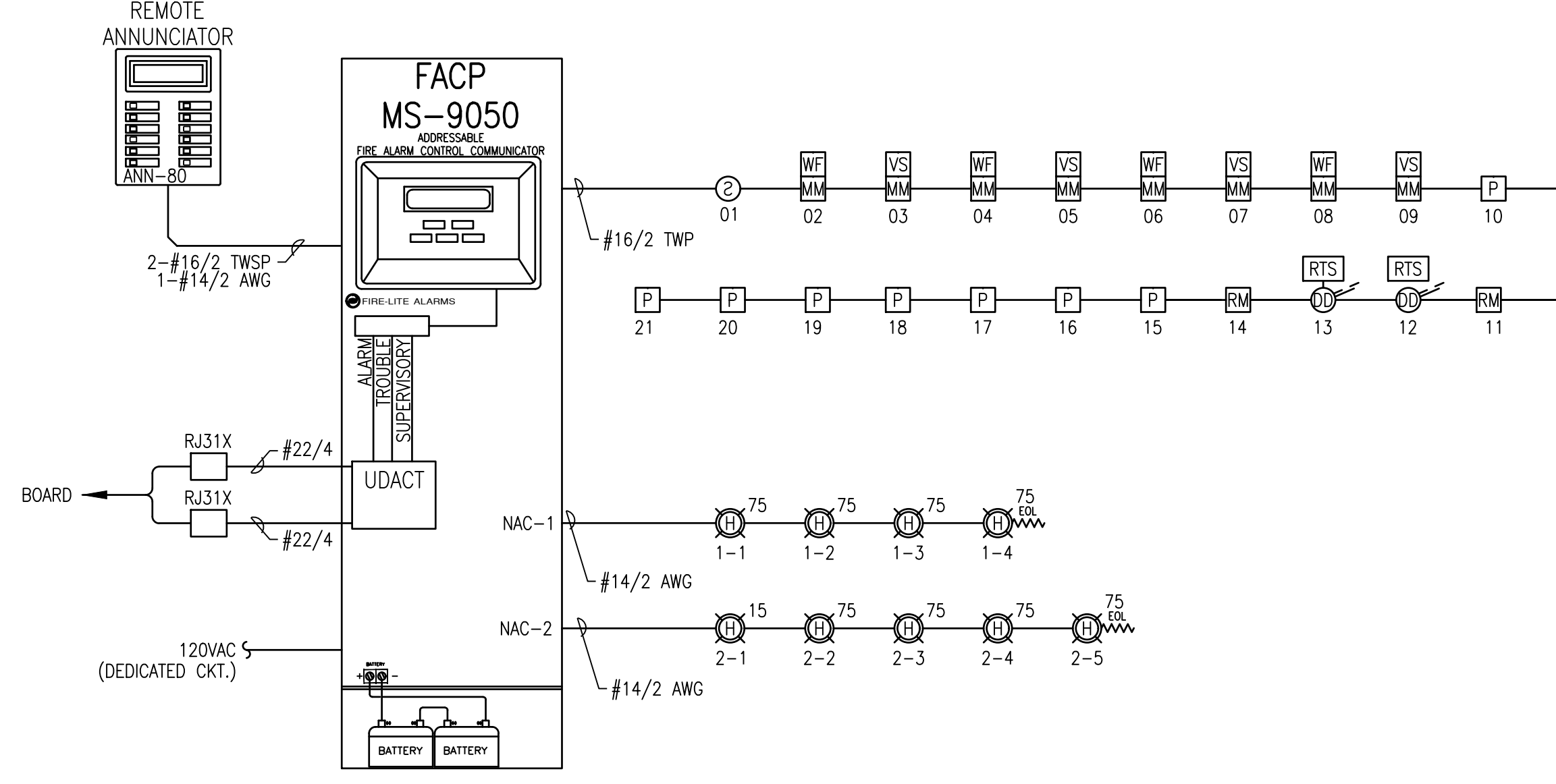
BUILDING B FIRE ALARM PLAN SCHEMATIC: NO SCALE
