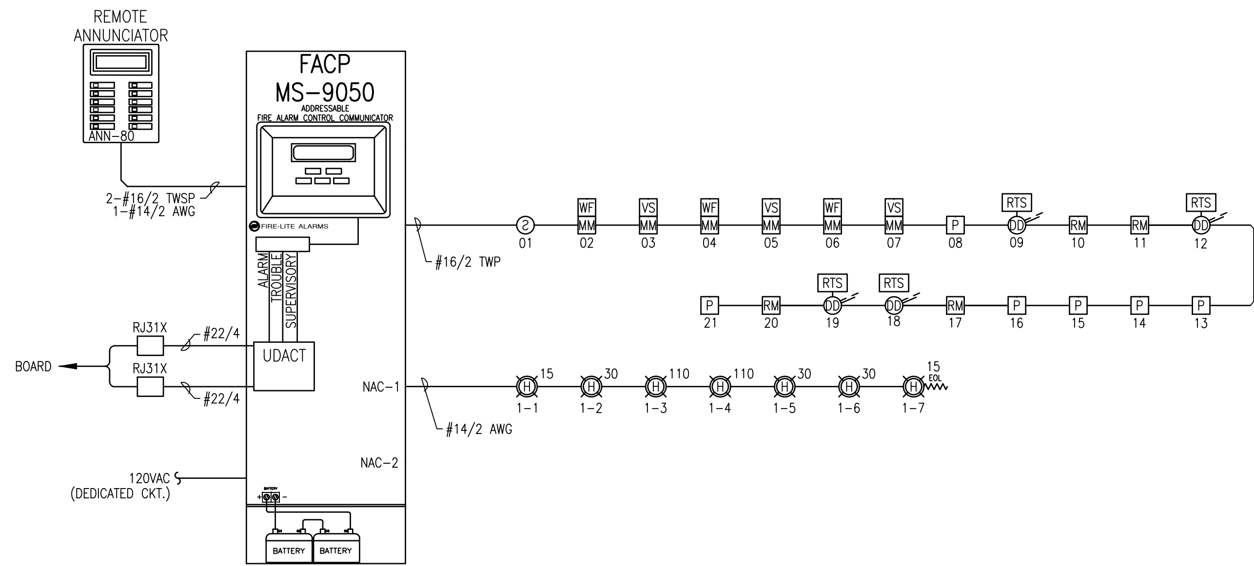
BUILDING A FIRE ALARM PLAN SCHEMATIC: NO SCALE
