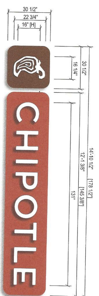
SIGN TYPE B-3 Sign Layout Detail Scale: 3/8" = 1'-0"
