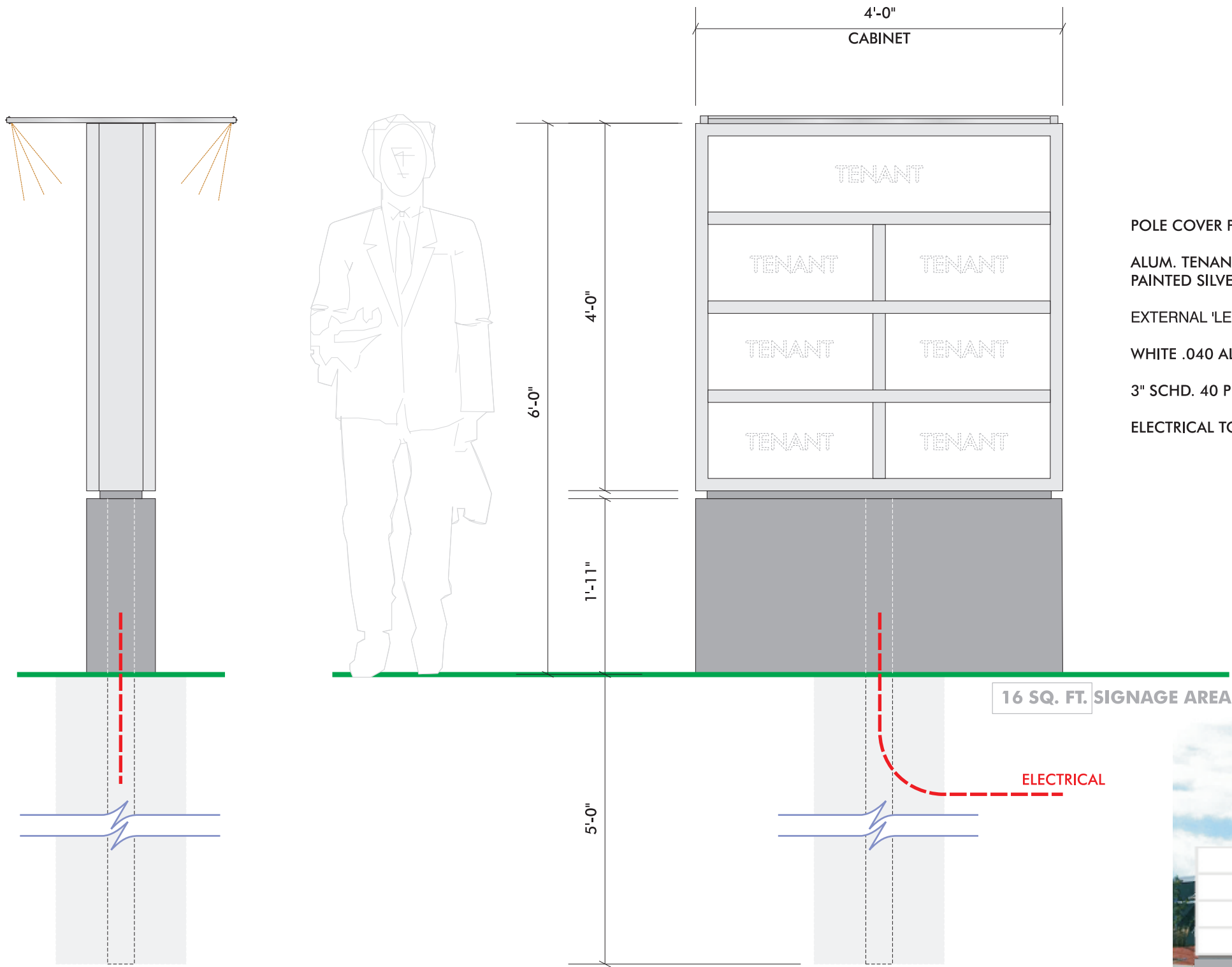
END VIEW
