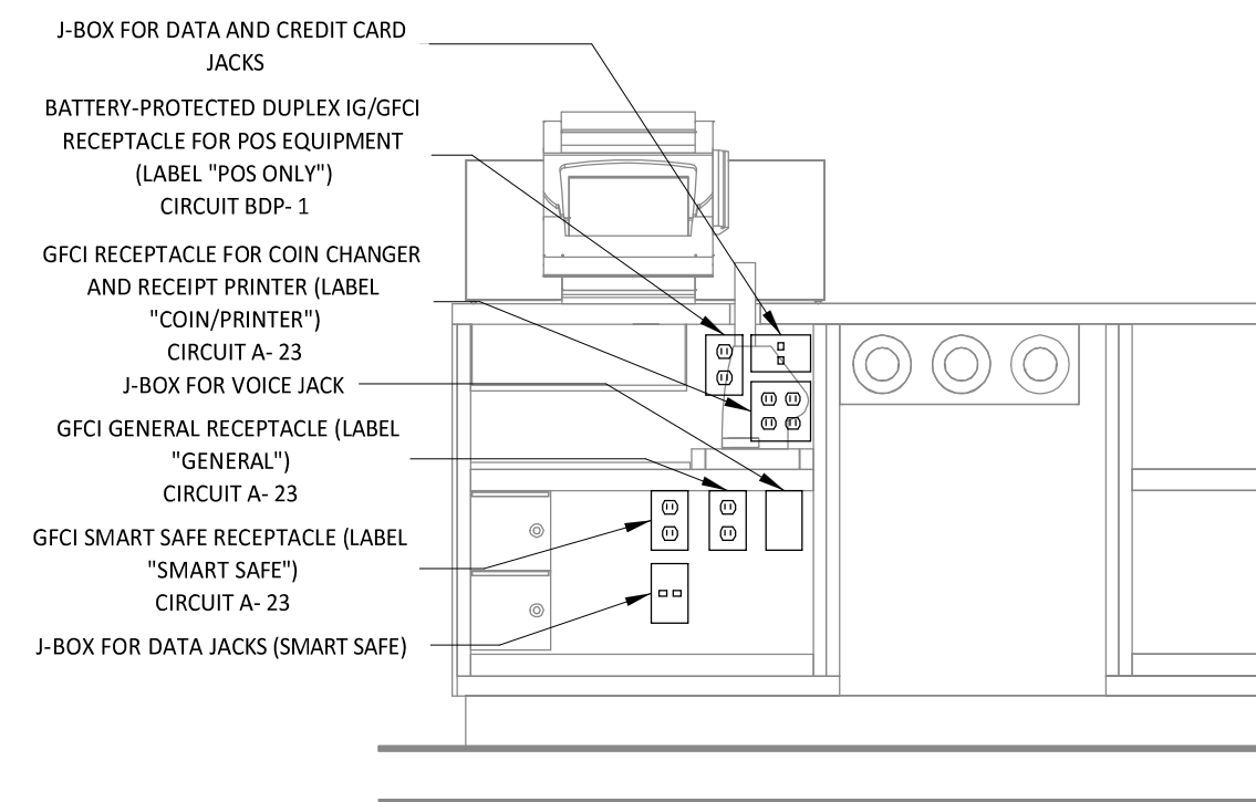
POS COUNTER ELECTRICAL ELEVATION E300 N.T.S.
