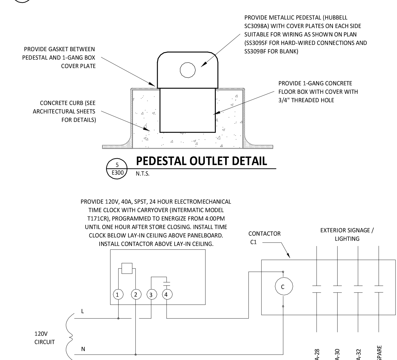
EXTERIOR SIGN LIGHTING CONTROL E300 N.T.S.
