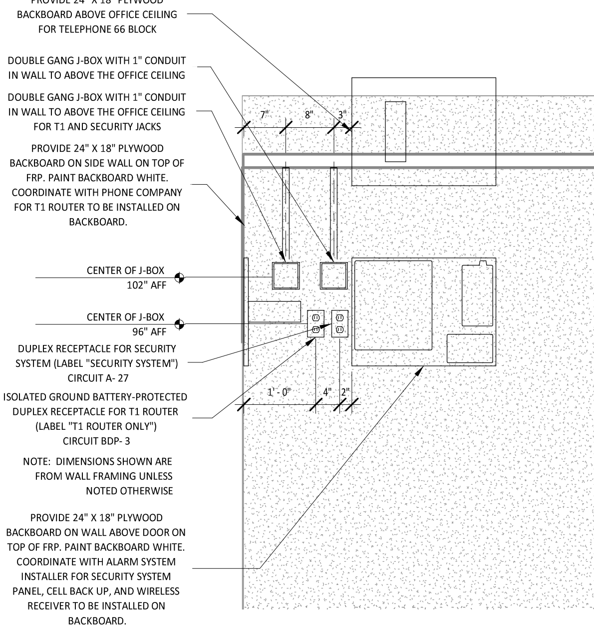
OFFICE EQUIPMENT ELECTRICAL ELEVATION E300 N.T.S.
