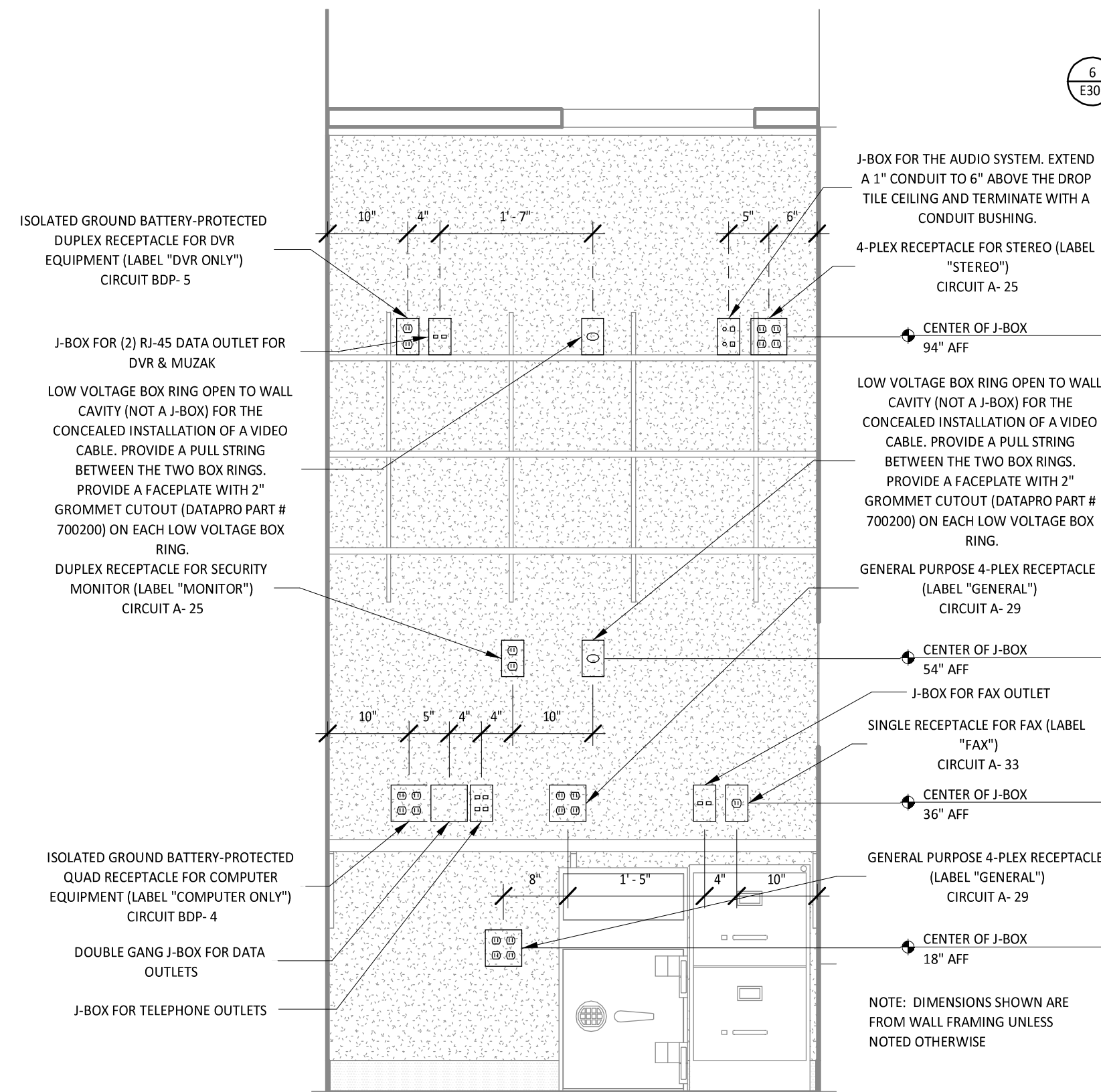
OFFICE DESK ELECTRICAL ELEVATION E300 N.T.S.
