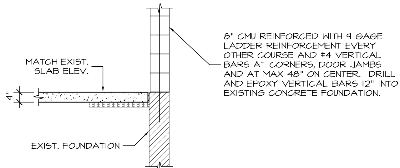
SECTION 9 1/2"=1'-0" S1.2
