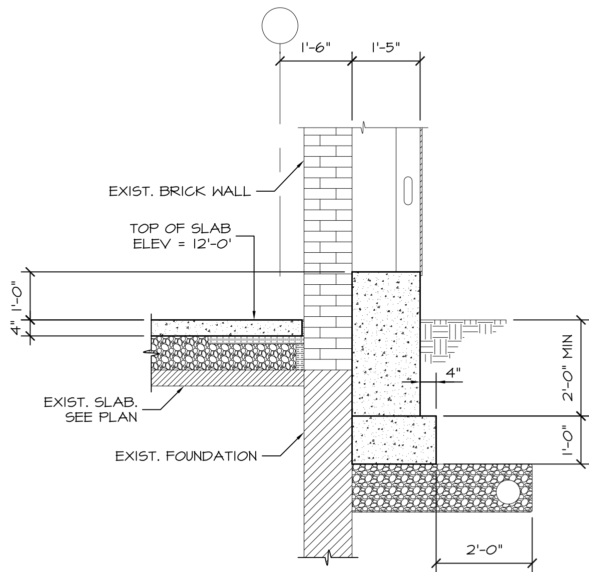
SECTION 4 1/2"=1'-0" S1.1
