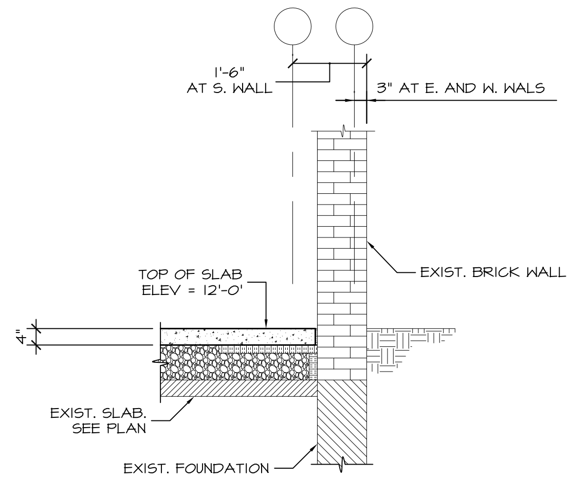
SECTION 3 1/2"=1'-0" S1.1
