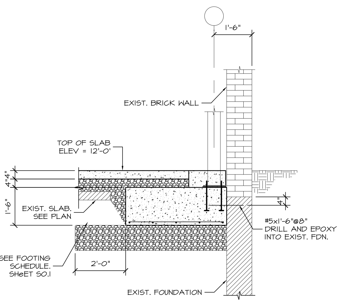
SECTION 7 1/2"=1'-0" S1.1
