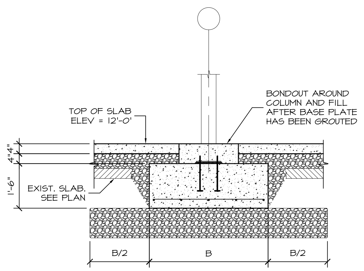
SECTION 8 1/2"=1'-0" S1.1
