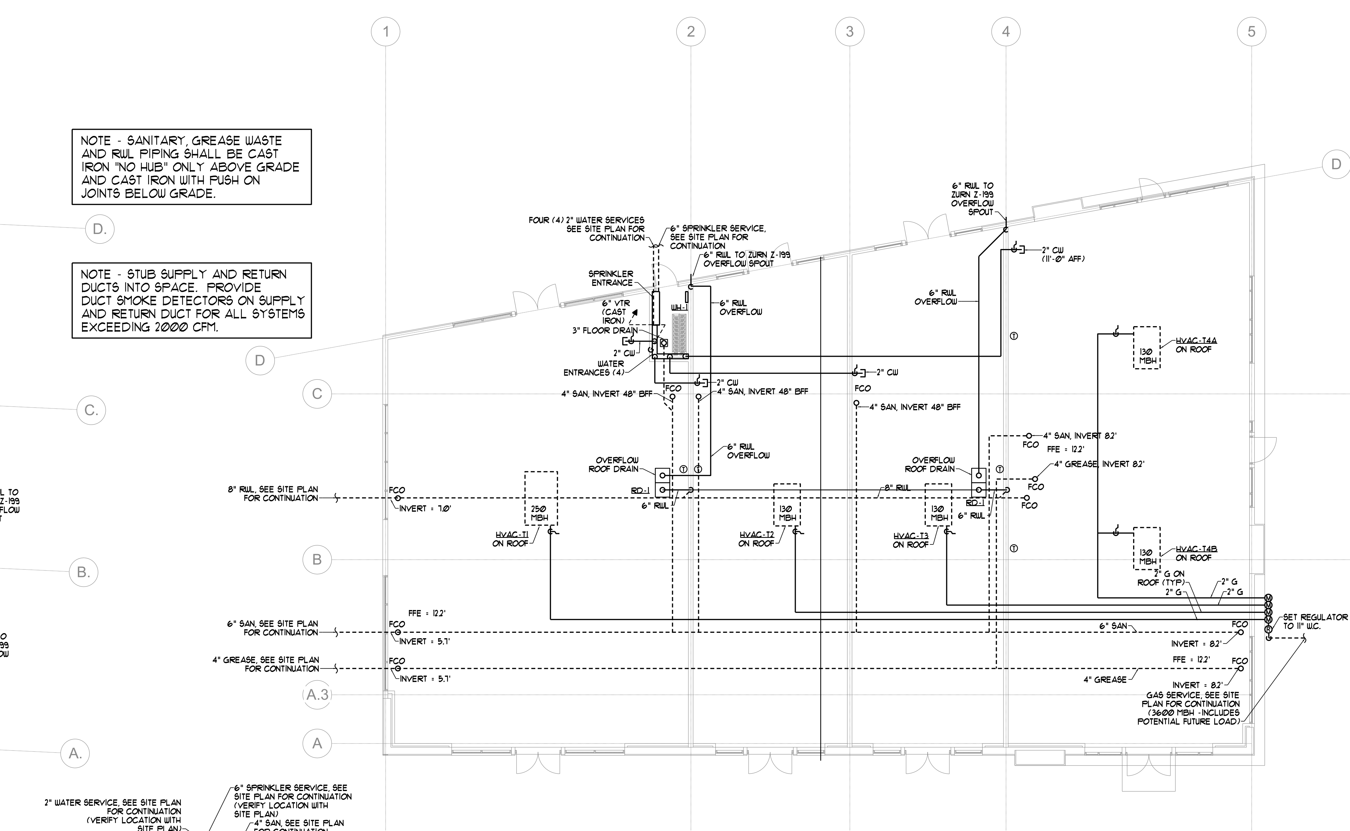
BUILDING B MECHANICAL AND PLUMBING PLAN SCALE - 1/8" = 1'-0"
