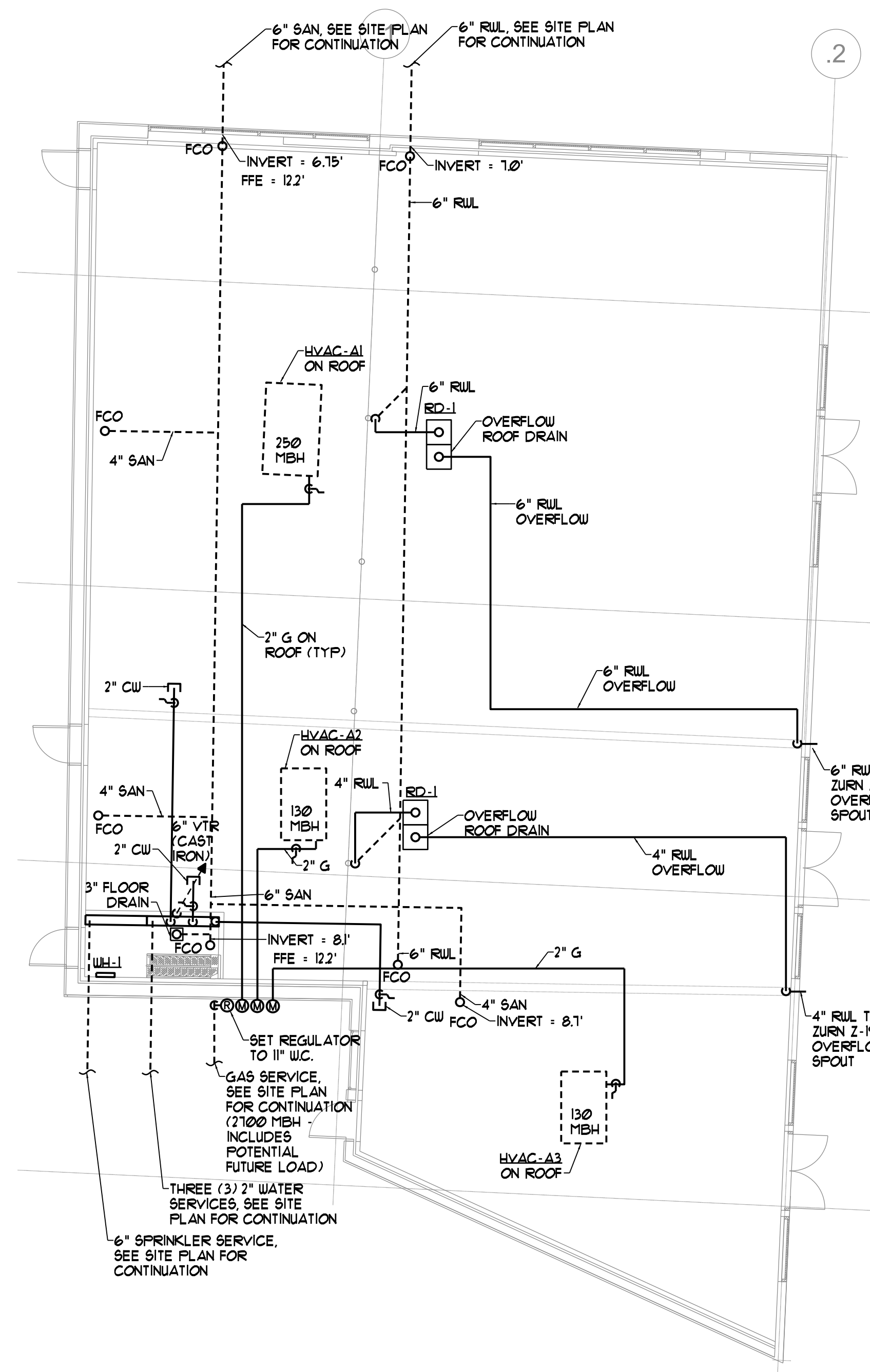
BUILDING A MECHANICAL AND PLUMBING PLAN SCALE - 1/8" = 1'-0"
