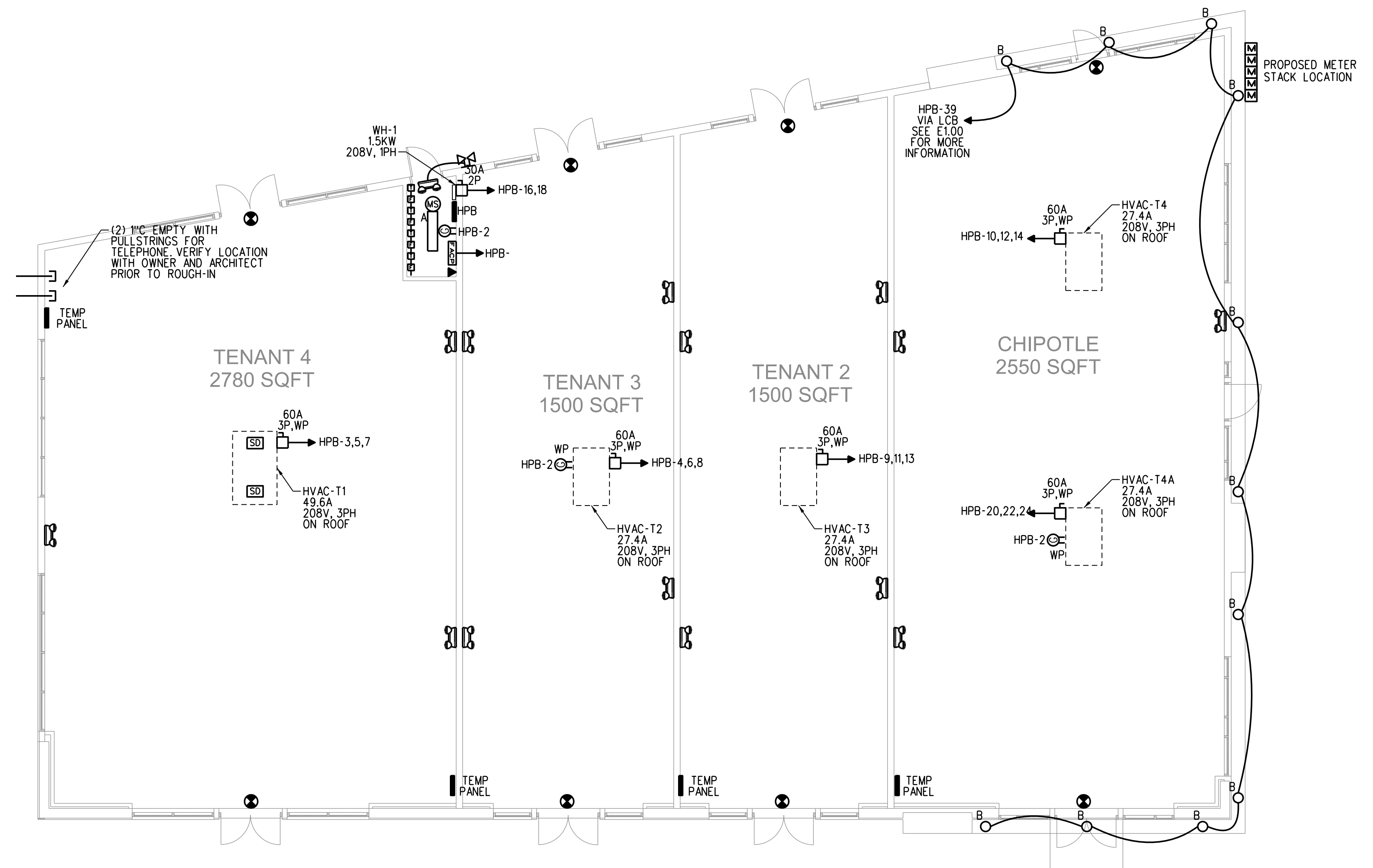
BUILDING B SHELL SCALE: 1/8"=1'-0"
