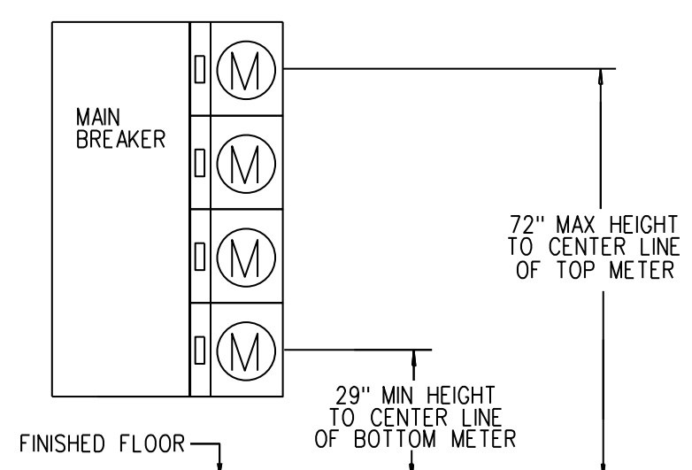
BUILDING A METER STACK ELEVATION (4 METERS TOTAL) SCALE: NONE
