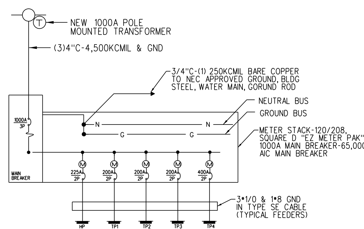
BUILDING B ONE-LINE DIAGRAM SCALE: NONE
