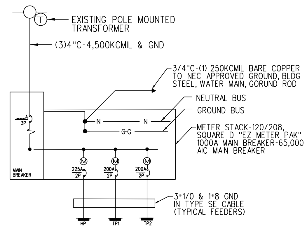
BUILDING A ONE-LINE DIAGRAM SCALE: NONE
