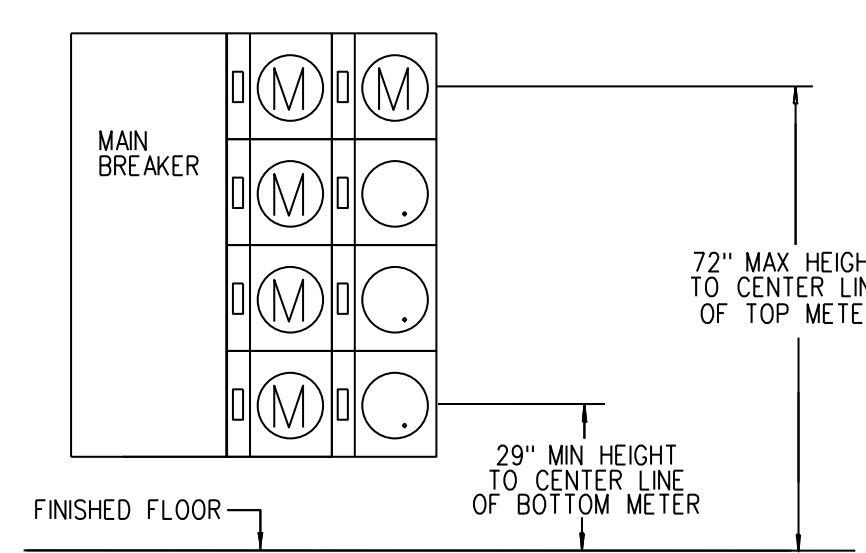
BUILDING B METER STACK ELEVATION (5 METERS TOTAL) SCALE: NONE
