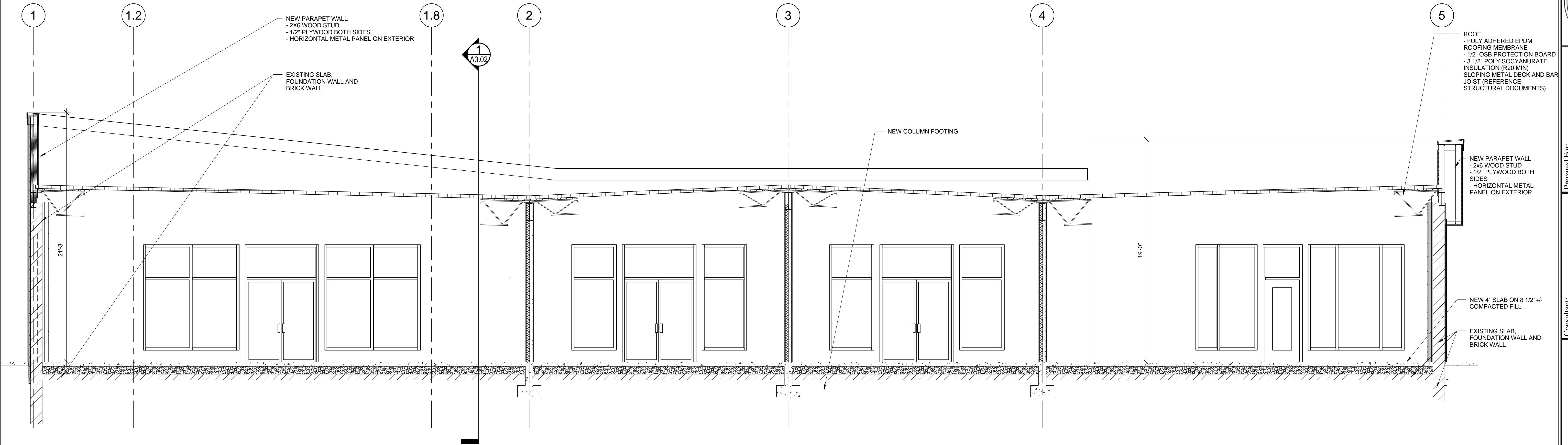
1 BUILDING B EAST-WEST SECTION THROUGH EXISTING BRICK WALLS
