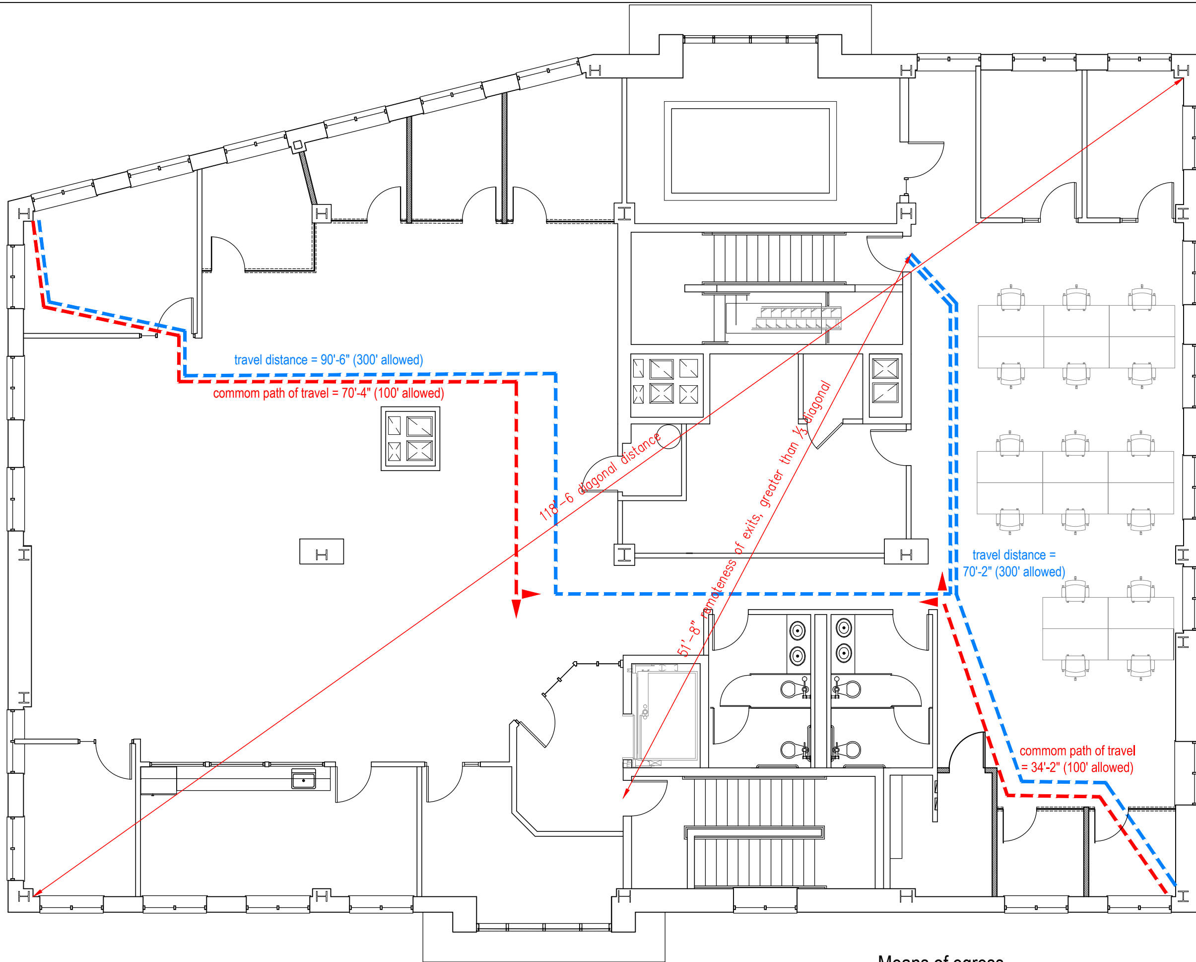
1 Means of egress 1/8" = 1'-0"
