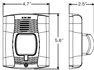
Wall-mount horn/strobes
