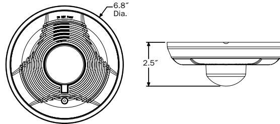
Ceiling-mount horn/strobes
