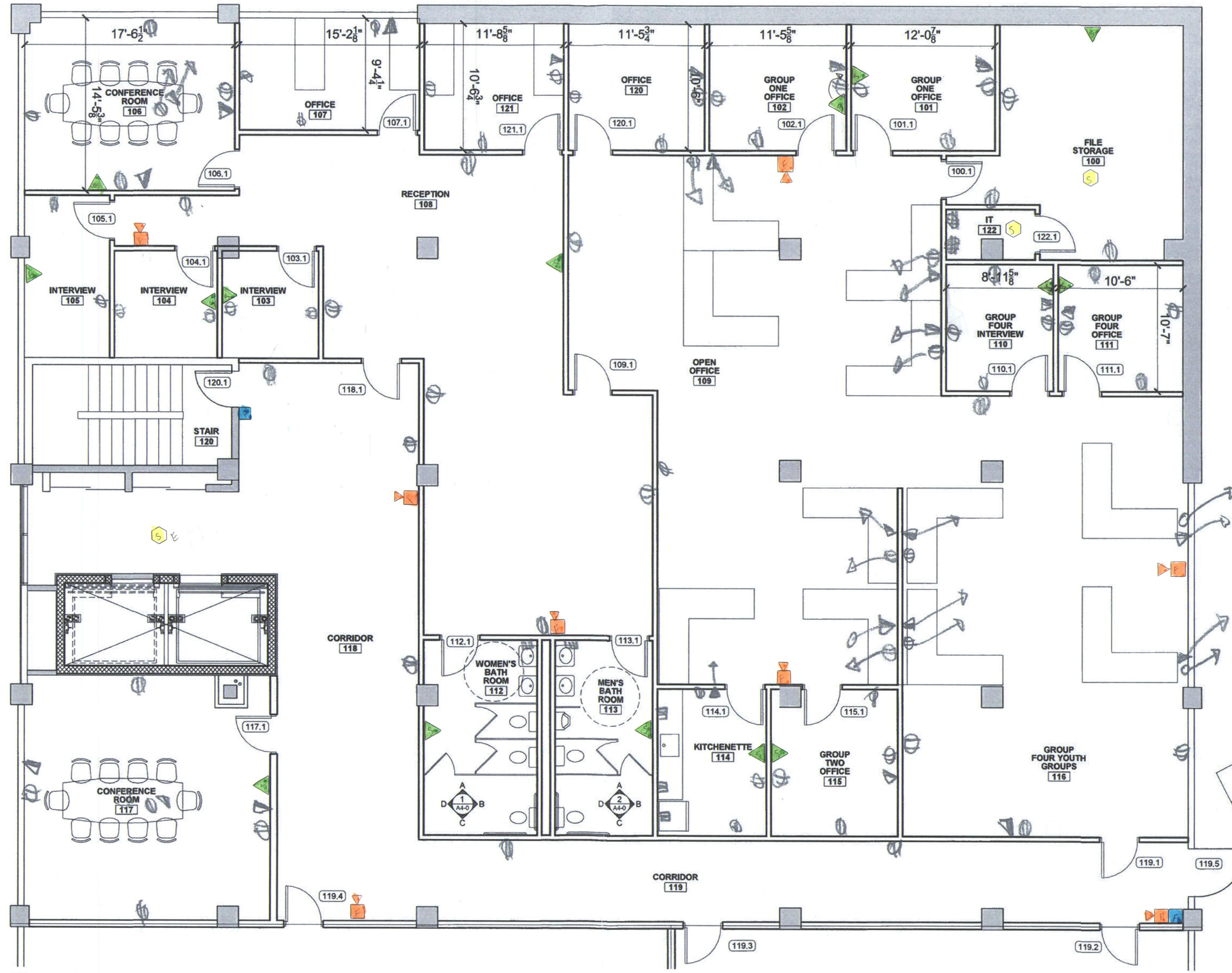
1 FIRST FLOOR PLAN 1/4" = 1'-0"
